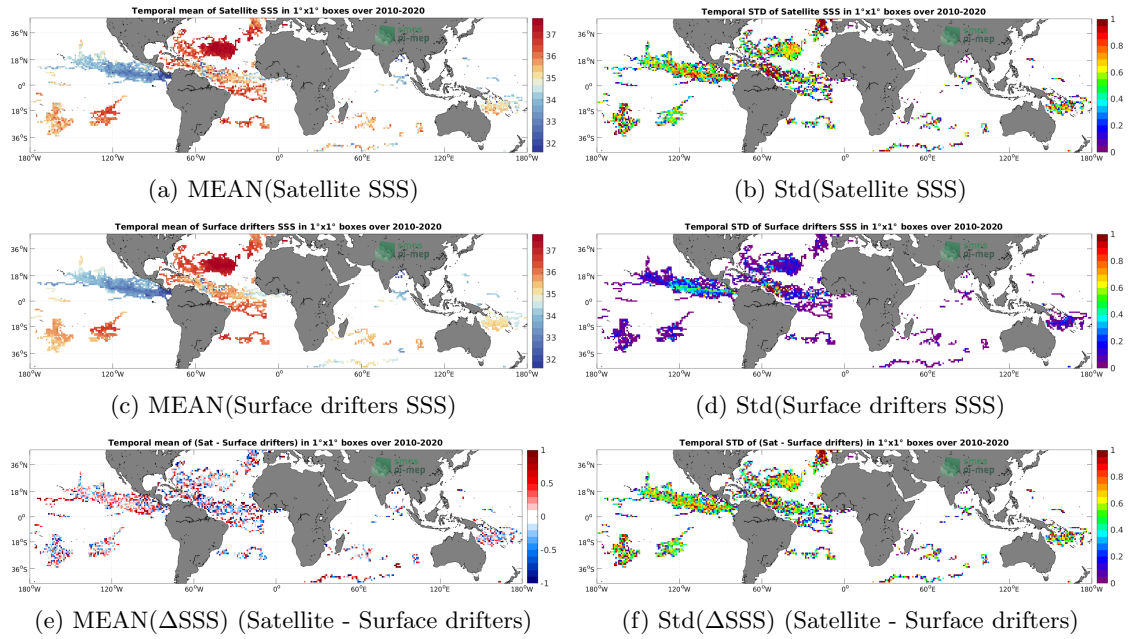
Figure 5: Temporal mean (left) and Std (right) of SSS from SMOS SSS L2Q v330 - 0.25 Deg (CATDS-CPDC) (top), Surface drifters (middle), and of \Delta SSS (Satellite - Surface drifters). Only match-up pairs are used to generate these maps.
