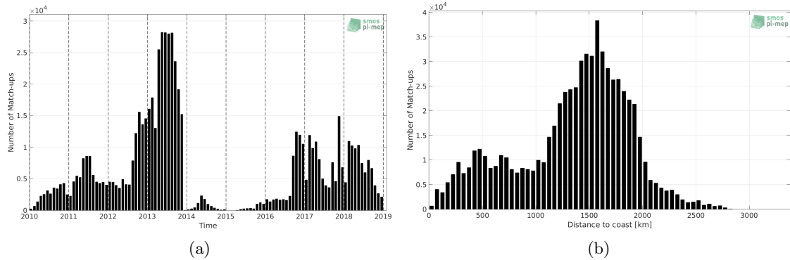
Figure 1: Number of match-ups between Surface drifters and SMOS SSS L2Q v330 - 0.25 Deg (CATDS-CPDC) SSS as a function of time (a) and as function of the distance to coast (b) over the Mid-Low Latitudes 45N-45S Pi-MEP region and for the full satellite product period.
