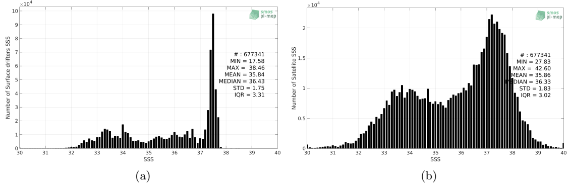
Figure 2: Histograms of SSS from Surface drifters (a) and SMOS SSS L2Q v330 - 0.25 Deg (CATDS-CPDC) (b) considering all match-up pairs per bins of 0.1 over the Mid-Low Latitudes 45N-45S Pi-MEP region and for the full satellite product period.
