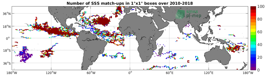
Figure 3: Number of SSS match-ups between Surface drifters SSS and the SMOS SSS L2Q v330 - 0.25 Deg (CATDS-CPDC) SSS product for the Mid-Low Latitudes 45N-45S Pi-MEP region over 1^\circ \times 1^\circ boxes and for the full satellite product period.
