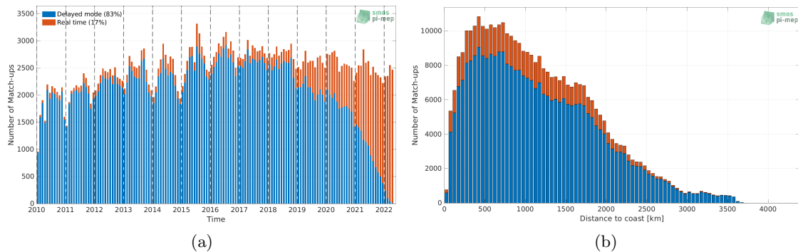
Figure 1: Number of match-ups between Argo and SMOS SSS L2Q v330 - 0.25 Deg (CATDS-CPDC) SSS as a function of time (a) and as function of the distance to coast (b) over the Mid-Low Latitudes 45N-45S Pi-MEP region and for the full satellite product period.
