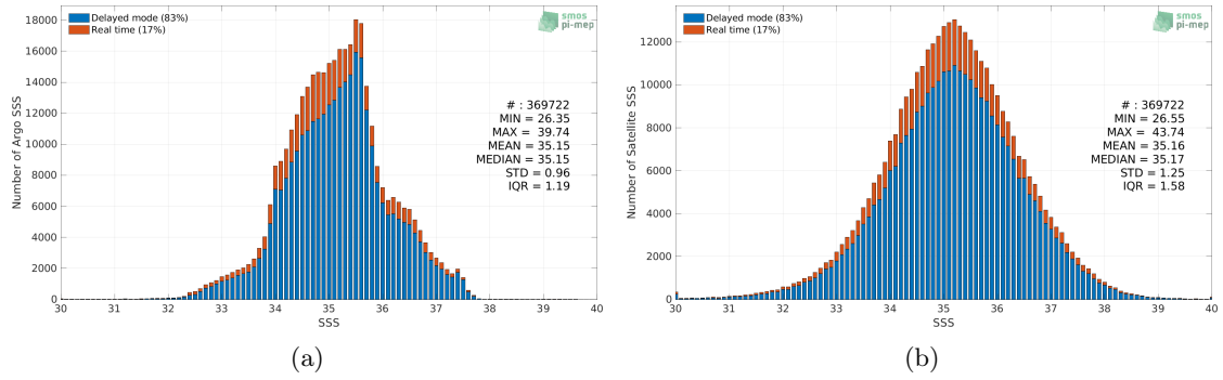
Figure 2: Histograms of SSS from Argo (a) and SMOS SSS L2Q v330 - 0.25 Deg (CATDS-CPDC) (b) considering all match-up pairs per bins of 0.1 over the Mid-Low Latitudes 45N-45S Pi-MEP region and for the full satellite product period.
