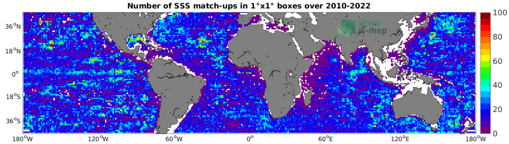
Figure 4: Number of SSS match-ups between Argo SSS and the SMOS SSS L2Q v330 - 0.25 Deg (CATDS-CPDC) SSS product for the Mid-Low Latitudes 45N-45S Pi-MEP region over 1^\circ \times 1^\circ boxes and for the full satellite product period.
