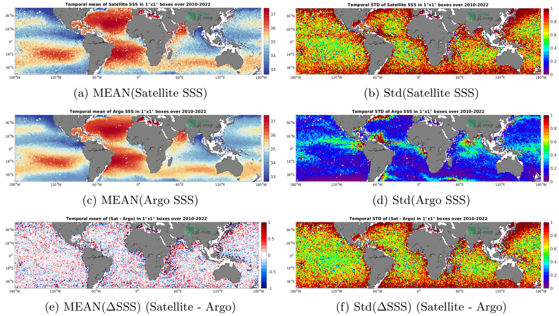
Figure 6: Temporal mean (left) and Std (right) of SSS from SMOS SSS L2Q v330 - 0.25 Deg (CATDS-CPDC) (top), Argo (middle), and of \Delta SSS (Satellite - Argo). Only match-up pairs are used to generate these maps.
