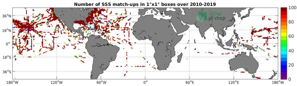
Figure 4: Number of SSS match-ups between TSG-SAMOS SSS and the SMOS-L3-CATDS-CPDC-V321-L2Q SSS product for the Mid-Low Latitudes 45N-45S Pi-MEP region over 1^\circ \times 1^\circ boxes and for the full satellite product period.
