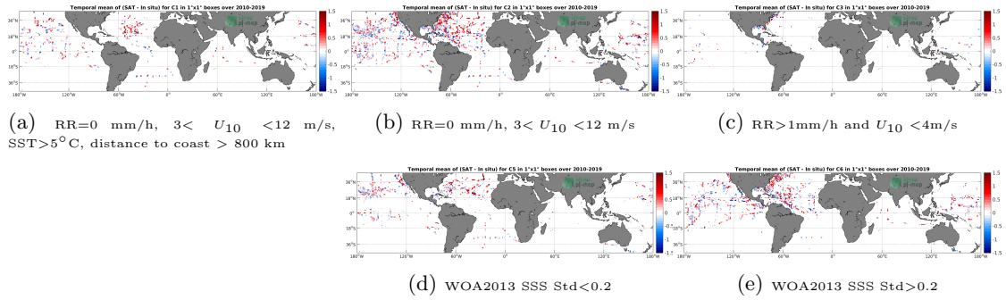
Figure 12: Temporal mean gridded over spatial boxes of size 1^\circ \times 1^\circ of \Delta SSS (SMOS-L3-CATDS-CPDC-V321-L2Q - TSG-SAMOS) for 5 different subdatasets corresponding to:RR=0 mm/h, 3 < U_{10} < 12 m/s, SST >5^\circ\text{C} , distance to coast > 800 km (a), RR=0 mm/h, 3 < U_{10} < 12 m/s (b), RR >1 mm/h and U_{10} < 4 m/s (c), WOA2013 SSS Std <0.2 (d), WOA2013 SSS Std >0.2 (e).
