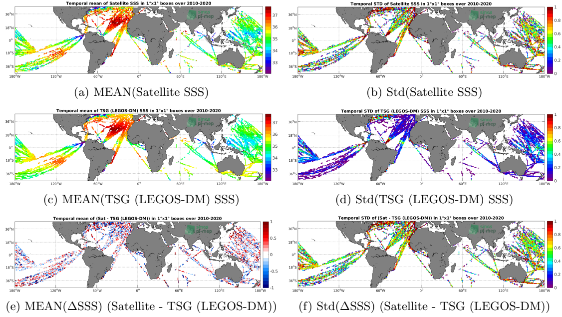
Figure 6: Temporal mean (left) and Std (right) of SSS from SMOS SSS L2Q v321 - 0.25 Deg (CATDS-CPDC) (top), TSG (LEGOS-DM) (middle), and of \Delta SSS (Satellite - TSG (LEGOS-DM)). Only match-up pairs are used to generate these maps.
