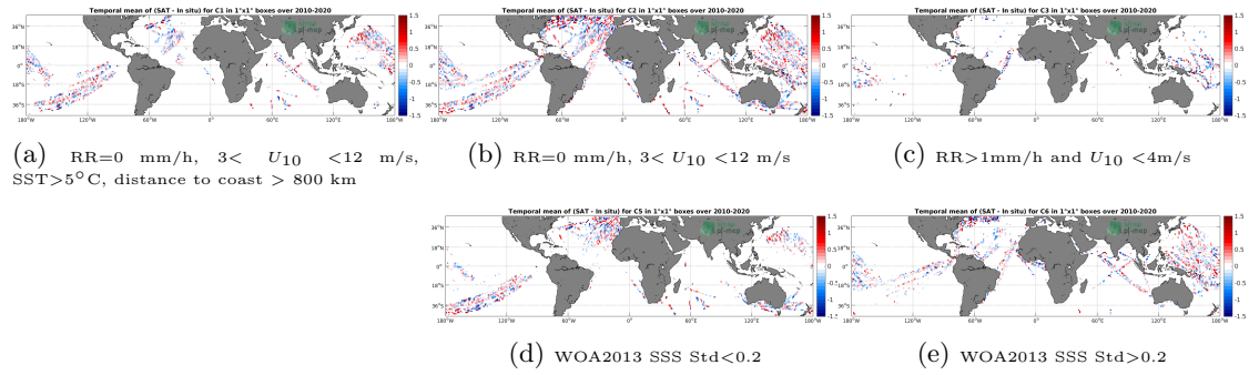
Figure 12: Temporal mean gridded over spatial boxes of size 1^\circ \times 1^\circ of \Delta SSS (SMOS SSS L2Q v321 - 0.25 Deg (CATDS-CPDC) - TSG (LEGOS-DM)) for 5 different subdatasets corresponding to: RR=0 mm/h, 3 < U_{10} < 12 m/s, SST > 5^\circ C , distance to coast > 800 km (a), RR=0 mm/h, 3 < U_{10} < 12 m/s (b), RR > 1 mm/h and U_{10} < 4 m/s (c), WOA2013 SSS Std < 0.2 (d), WOA2013 SSS Std > 0.2 (e).
