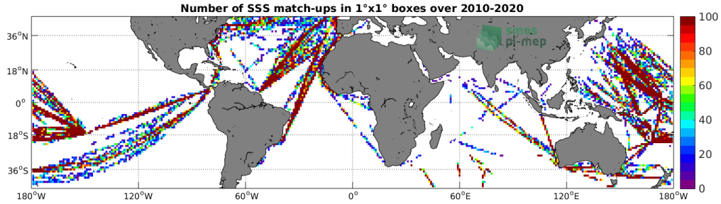
Figure 4: Number of SSS match-ups between TSG (LEGOS-DM) SSS and the SMOS SSS L2Q v321 - 0.25 Deg (CATDS-CPDC) SSS product for the Mid-Low Latitudes 45N-45S Pi-MEP region over 1^\circ \times 1^\circ boxes and for the full satellite product period.
