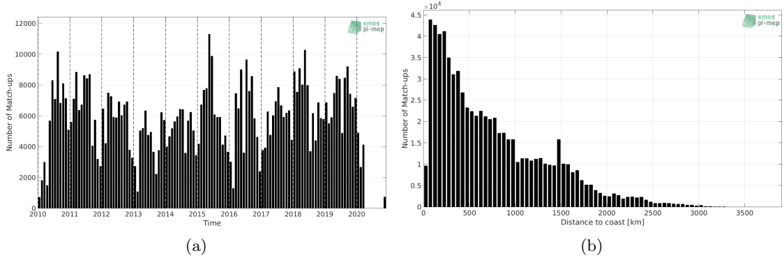
Figure 1: Number of match-ups between TSG (LEGOS-DM) and SMOS SSS L2Q v321 - 0.25 Deg (CATDS-CPDC) SSS as a function of time (a) and as function of the distance to coast (b) over the Mid-Low Latitudes 45N-45S Pi-MEP region and for the full satellite product period.
