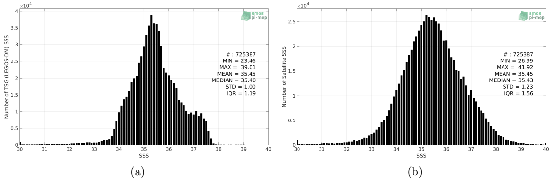
Figure 2: Histograms of SSS from TSG (LEGOS-DM) (a) and SMOS SSS L2Q v321 - 0.25 Deg (CATDS-CPDC) (b) considering all match-up pairs per bins of 0.1 over the Mid-Low Latitudes 45N-45S Pi-MEP region and for the full satellite product period.
