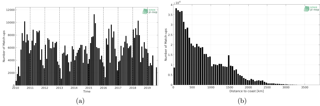
Figure 1: Number of match-ups between TSG-LEGOS-DM and SMOS L2Q v321 - 0.25 Deg (CATDS-CPDC) SSS as a function of time (a) and as function of the distance to coast (b) over the Mid-Low Latitudes 45N-45S Pi-MEP region and for the full satellite product period.
