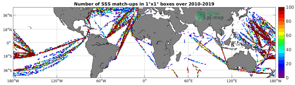
Figure 4: Number of SSS match-ups between TSG-LEGOS-DM SSS and the SMOS L2Q v321 - 0.25 Deg (CATDS-CPDC) SSS product for the Mid-Low Latitudes 45N-45S Pi-MEP region over 1^\circ \times 1^\circ boxes and for the full satellite product period.
