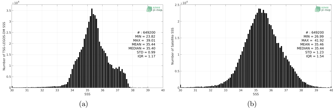
Figure 2: Histograms of SSS from TSG-LEGOS-DM (a) and SMOS L2Q v321 - 0.25 Deg (CATDS-CPDC) (b) considering all match-up pairs per bins of 0.1 over the Mid-Low Latitudes 45N-45S Pi-MEP region and for the full satellite product period.
