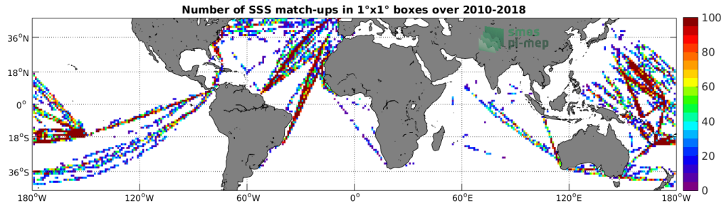
Figure 4: Number of SSS match-ups between TSG-LEGOS-DM SSS and the SMOS-L3-CATDS-CPDC-V321-L2Q SSS product for the Mid-Low Latitudes 45N-45S Pi-MEP region over 1^\circ \times 1^\circ boxes and for the full satellite product period.
