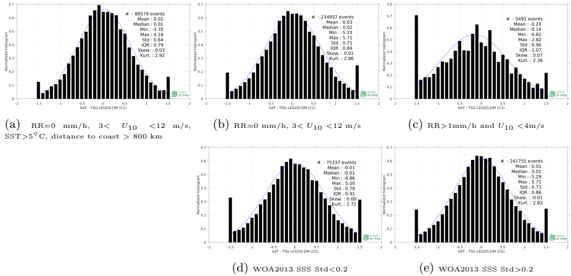
Figure 13: Normalized histogram of \Delta SSS (SMOS-L3-CATDS-CPDC-V321-L2Q - TSG-LEGOS-DM) for 5 different subdatasets corresponding to: RR=0 mm/h, 3 < U_{10} < 12 m/s, SST > 5^\circ C , distance to coast > 800 km (a), RR=0 mm/h, 3 < U_{10} < 12 m/s (b), RR > 1 mm/h and U_{10} < 4 m/s (c), WOA2013 SSS Std < 0.2 (d), WOA2013 SSS Std > 0.2 (e).
