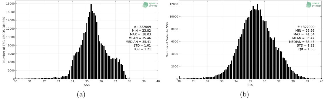
Figure 2: Histograms of SSS from TSG-LEGOS-DM (a) and SMOS-L3-CATDS-CPDC-V321-L2Q (b) considering all match-up pairs per bins of 0.1 over the Mid-Low Latitudes 45N-45S Pi-MEP region and for the full satellite product period.
