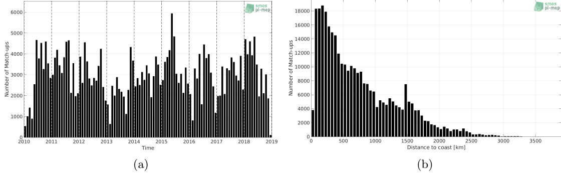
Figure 1: Number of match-ups between TSG-LEGOS-DM and SMOS-L3-CATDS-CPDC-V321-L2Q SSS as a function of time (a) and as function of the distance to coast (b) over the Mid-Low Latitudes 45N-45S Pi-MEP region and for the full satellite product period.
