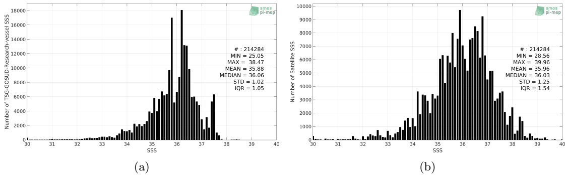
Figure 2: Histograms of SSS from TSG-GOSUD-Research-vessel (a) and SMOS-L3-CATDS-CPDC-V321-L2Q (b) considering all match-up pairs per bins of 0.1 over the Mid-Low Latitudes 45N-45S Pi-MEP region and for the full satellite product period.
