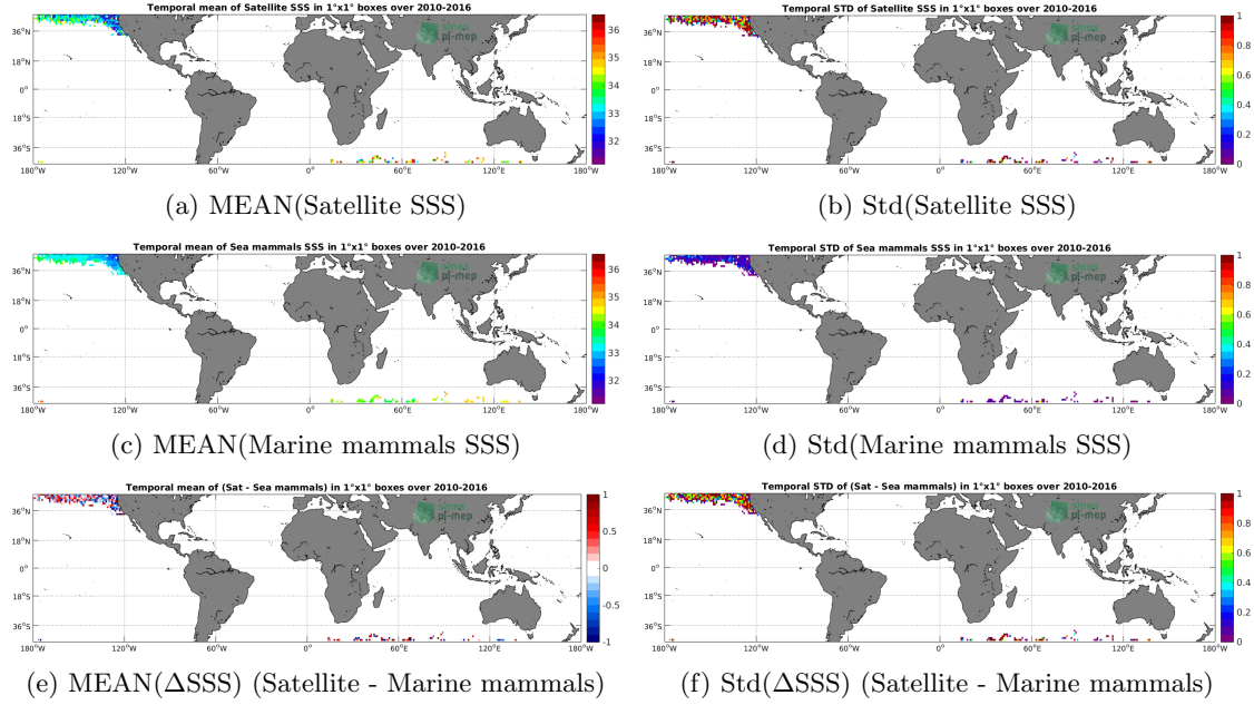
Figure 6: Temporal mean (left) and Std (right) of SSS from SMOS SSS L2Q v321 - 0.25 Deg (CATDS-CPDC) (top), Marine mammals (middle), and of \Delta SSS (Satellite - Marine mammals). Only match-up pairs are used to generate these maps.
