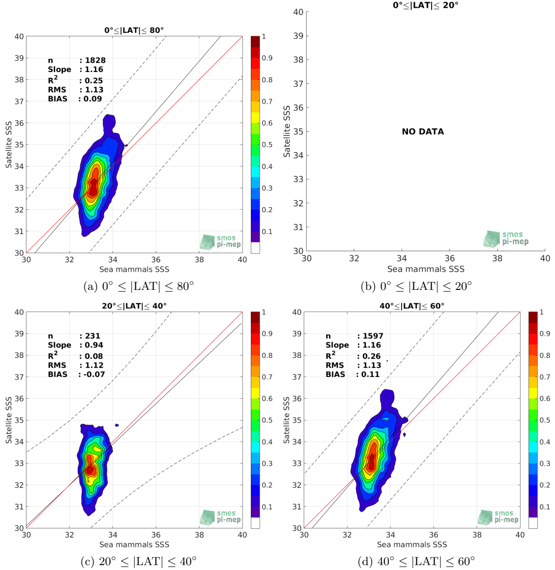
Figure 9: Contour maps of the concentration of SMOS SSS L2Q v321 - 0.25 Deg (CATDS-CPDC) SSS (y-axis) versus Marine mammals SSS (x-axis) at match-up pairs for different latitude bands. For each plot, the red line shows x=y . The black thin and dashed lines indicate a linear fit through the data cloud and the \pm 95\% confidence levels, respectively. The number match-up pairs n , the slope and R^2 coefficient of the linear fit, the root mean square (RMS) and the mean bias between satellite and in situ data are indicated for each latitude band in each plots.
