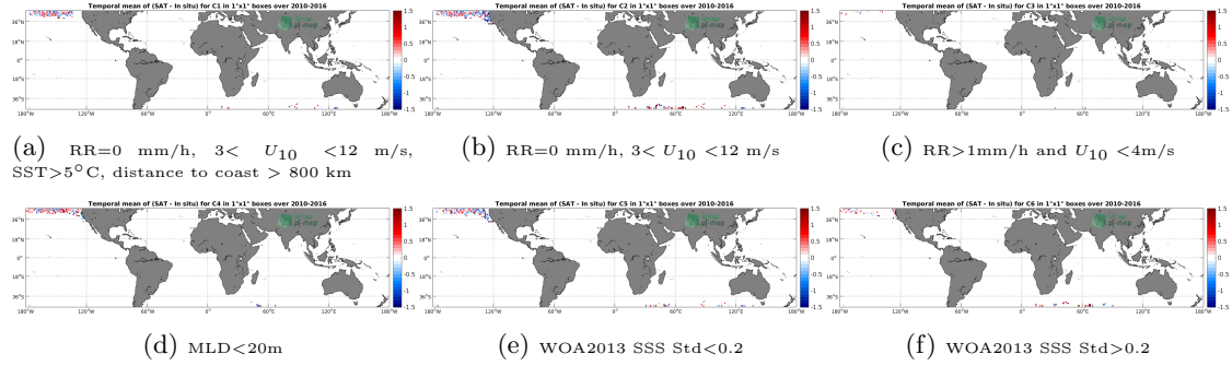
Figure 12: Temporal mean gridded over spatial boxes of size 1^\circ \times 1^\circ of \Delta SSS (SMOS SSS L2Q v321 - 0.25 Deg (CATDS-CPDC) - Marine mammals) for 6 different subdatasets corresponding to: RR=0 mm/h, 3 < U_{10} < 12 m/s, SST > 5^\circ C , distance to coast > 800 km (a), RR=0 mm/h, 3 < U_{10} < 12 m/s (b), RR > 1 mm/h and U_{10} < 4 m/s (c), MLD < 20 m (d), WOA2013 SSS Std < 0.2 (e), WOA2013 SSS Std > 0.2 (f).
