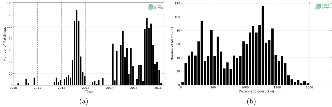
Figure 1: Number of match-ups between Marine mammals and SMOS SSS L2Q v321 - 0.25 Deg (CATDS-CPDC) SSS as a function of time (a) and as function of the distance to coast (b) over the Mid-Low Latitudes 45N-45S Pi-MEP region and for the full satellite product period.
