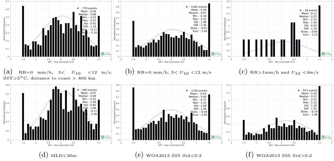
Figure 13: Normalized histogram of \Delta SSS (SMOS SSS L2Q v321 - 0.25 Deg (CATDS-CPDC) - Marine mammals) for 6 different subdatasets corresponding to: RR=0 mm/h, 3 < U_{10} < 12 m/s, SST>5°C, distance to coast > 800 km (a), RR=0 mm/h, 3 < U_{10} < 12 m/s (b), RR>1mm/h and U_{10} < 4 m/s (c), MLD<20m (d), WOA2013 SSS Std<0.2 (e), WOA2013 SSS Std>0.2 (f).
