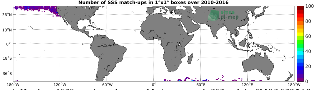
Figure 4: Number of SSS match-ups between Marine mammals SSS and the SMOS SSS L2Q v321 - 0.25 Deg (CATDS-CPDC) SSS product for the Mid-Low Latitudes 45N-45S Pi-MEP region over 1^\circ \times 1^\circ boxes and for the full satellite product period.
