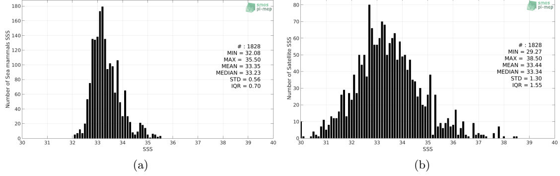
Figure 2: Histograms of SSS from Marine mammals (a) and SMOS SSS L2Q v321 - 0.25 Deg (CATDS-CPDC) (b) considering all match-up pairs per bins of 0.1 over the Mid-Low Latitudes 45N-45S Pi-MEP region and for the full satellite product period.
