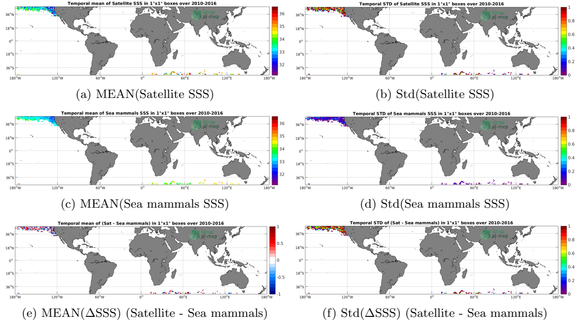
Figure 6: Temporal mean (left) and Std (right) of SSS from SMOS SSS L2Q v321 - 0.25 Deg (CATDS-CPDC) (top), Sea mammals (middle), and of \Delta SSS (Satellite - Sea mammals). Only match-up pairs are used to generate these maps.
