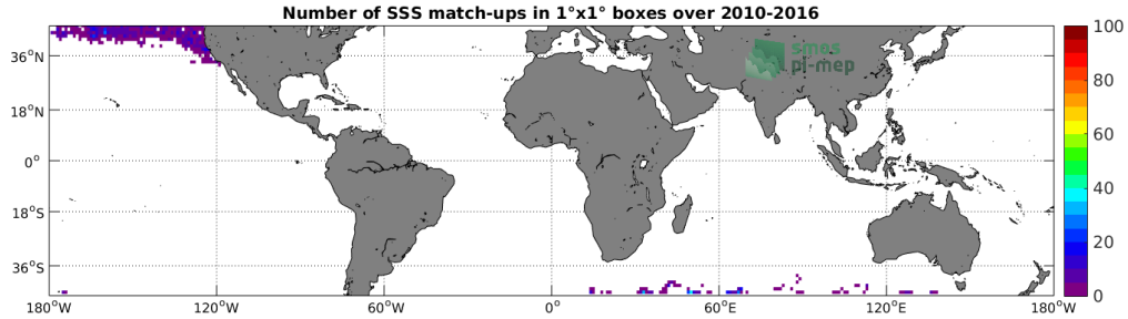
Figure 4: Number of SSS match-ups between Sea mammals SSS and the SMOS SSS L2Q v321 - 0.25 Deg (CATDS-CPDC) SSS product for the Mid-Low Latitudes 45N-45S Pi-MEP region over 1^\circ \times 1^\circ boxes and for the full satellite product period.
