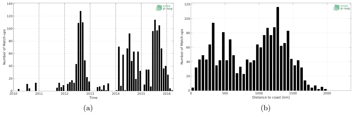
Figure 1: Number of match-ups between Sea mammals and SMOS SSS L2Q v321 - 0.25 Deg (CATDS-CPDC) SSS as a function of time (a) and as function of the distance to coast (b) over the Mid-Low Latitudes 45N-45S Pi-MEP region and for the full satellite product period.
