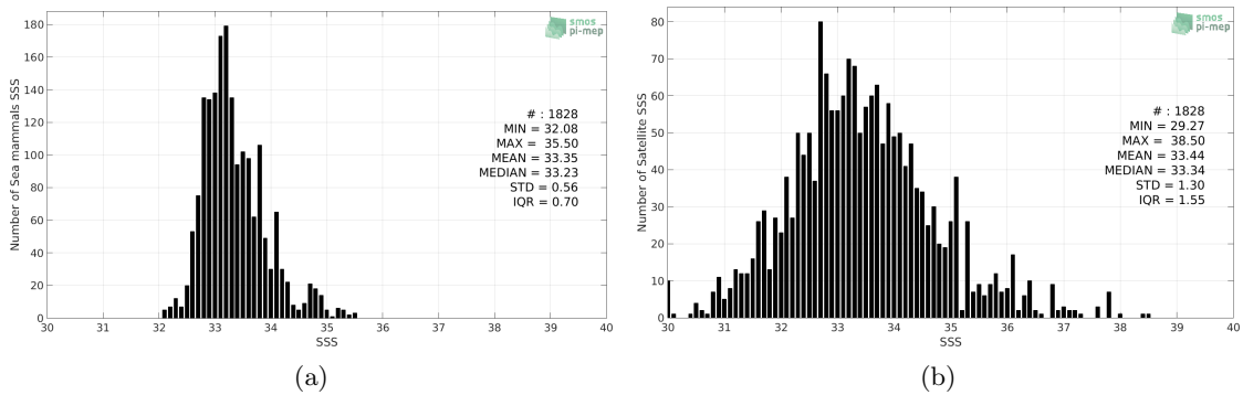
Figure 2: Histograms of SSS from Sea mammals (a) and SMOS SSS L2Q v321 - 0.25 Deg (CATDS-CPDC) (b) considering all match-up pairs per bins of 0.1 over the Mid-Low Latitudes 45N-45S Pi-MEP region and for the full satellite product period.
