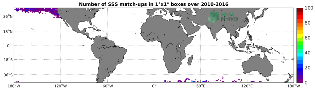
Figure 4: Number of SSS match-ups between Sea mammals SSS and the SMOS SSS L2Q v321 - 0.25 Deg (CATDS-CPDC) SSS product for the Mid-Low Latitudes 45N-45S Pi-MEP region over 1°x1° boxes and for the full satellite product period.
