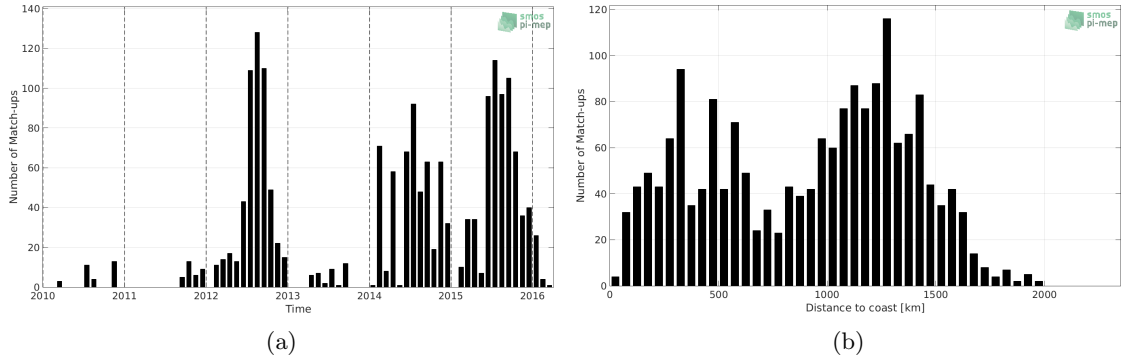
Figure 1: Number of match-ups between Sea mammals and SMOS SSS L2Q v321 - 0.25 Deg (CATDS-CPDC) SSS as a function of time (a) and as function of the distance to coast (b) over the Mid-Low Latitudes 45N-45S Pi-MEP region and for the full satellite product period.
