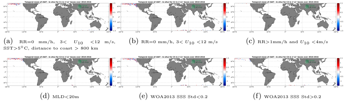
Figure 12: Temporal mean gridded over spatial boxes of size 1^\circ \times 1^\circ of \Delta SSS (SMOS-L3-CATDS-CPDC-V321-L2Q - Sea mammals) for 6 different subdatasets corresponding to: RR=0 mm/h, 3 < U_{10} < 12 m/s, SST > 5^\circ C , distance to coast > 800 km (a), RR=0 mm/h, 3 < U_{10} < 12 m/s (b), RR > 1 mm/h and U_{10} < 4 m/s (c), MLD < 20 m (d), WOA2013 SSS Std < 0.2 (e), WOA2013 SSS Std > 0.2 (f).
