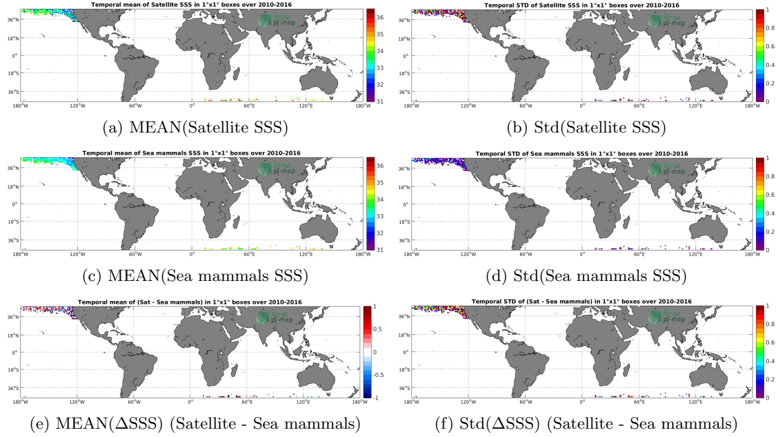
Figure 6: Temporal mean (left) and Std (right) of SSS from SMOS-L3-CATDS-CPDC-V321-L2Q (top), Sea mammals (middle), and of \Delta SSS (Satellite - Sea mammals). Only match-up pairs are used to generate these maps.
