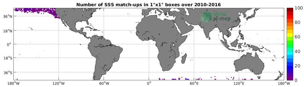
Figure 4: Number of SSS match-ups between Sea mammals SSS and the SMOS-L3-CATDS-CPDC-V321-L2Q SSS product for the Mid-Low Latitudes 45N-45S Pi-MEP region over 1°x1° boxes and for the full satellite product period.
