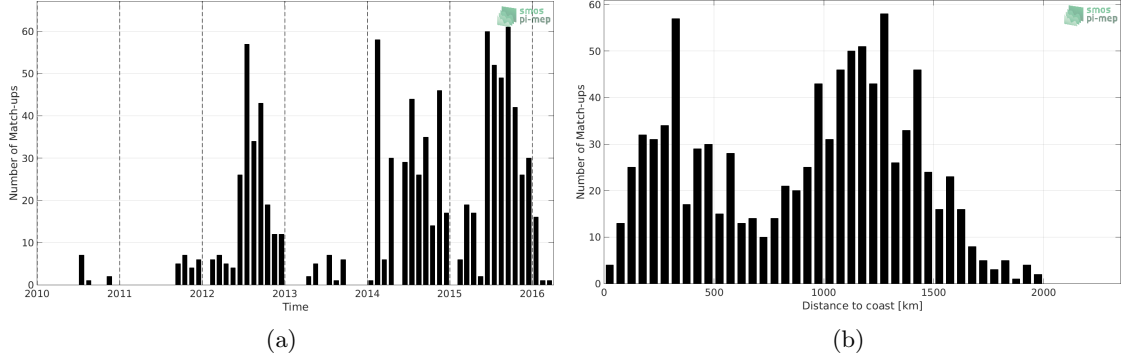
Figure 1: Number of match-ups between Sea mammals and SMOS-L3-CATDS-CPDC-V321-L2Q SSS as a function of time (a) and as function of the distance to coast (b) over the Mid-Low Latitudes 45N-45S Pi-MEP region and for the full satellite product period.
