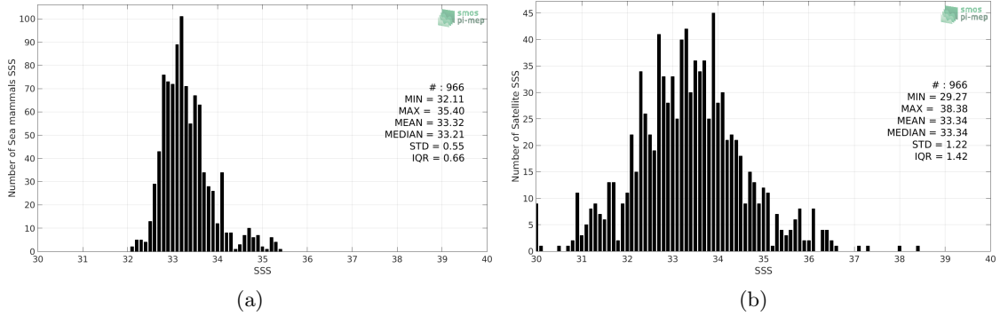
Figure 2: Histograms of SSS from Sea mammals (a) and SMOS-L3-CATDS-CPDC-V321-L2Q (b) considering all match-up pairs per bins of 0.1 over the Mid-Low Latitudes 45N-45S Pi-MEP region and for the full satellite product period.
