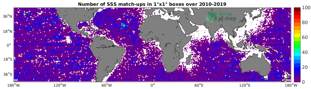
Figure 4: Number of SSS match-ups between Argo SSS and the SMOS-L3-CATDS-CPDC-V321-L2Q SSS product for the Mid-Low Latitudes 45N-45S Pi-MEP region over 1^\circ \times 1^\circ boxes and for the full satellite product period.
