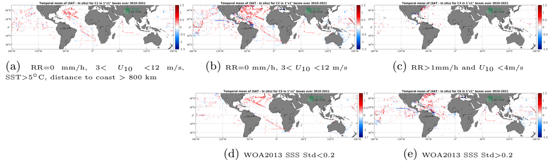
Figure 12: Temporal mean gridded over spatial boxes of size 1^\circ \times 1^\circ of \Delta SSS (SMOS SSS L3 v317 - Monthly - 25 km (CATDS-CPDC) - TSG (SAMOS)) for 5 different subdatasets corresponding to: RR=0 mm/h, 3 < U_{10} < 12 m/s, SST > 5^\circ C , distance to coast > 800 km (a), RR=0 mm/h, 3 < U_{10} < 12 m/s (b), RR > 1 mm/h and U_{10} < 4 m/s (c), WOA2013 SSS Std < 0.2 (d), WOA2013 SSS Std > 0.2 (e).
