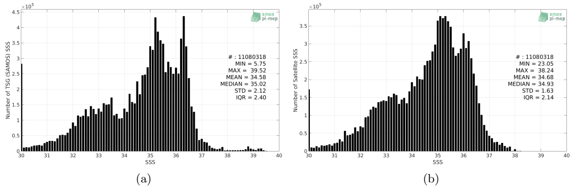
Figure 2: Histograms of SSS from TSG (SAMOS) (a) and SMOS SSS L3 v317 - Monthly - 25 km (CATDS-CPDC) (b) considering all match-up pairs per bins of 0.1 over the Mid-Low Latitudes 45N-45S Pi-MEP region and for the full satellite product period.
