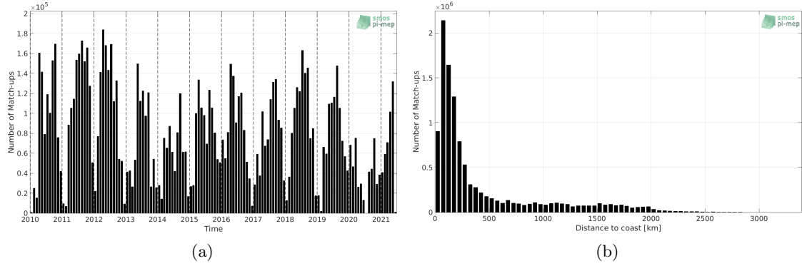
Figure 1: Number of match-ups between TSG (SAMOS) and SMOS SSS L3 v317 - Monthly - 25 km (CATDS-CPDC) SSS as a function of time (a) and as function of the distance to coast (b) over the Mid-Low Latitudes 45N-45S Pi-MEP region and for the full satellite product period.
