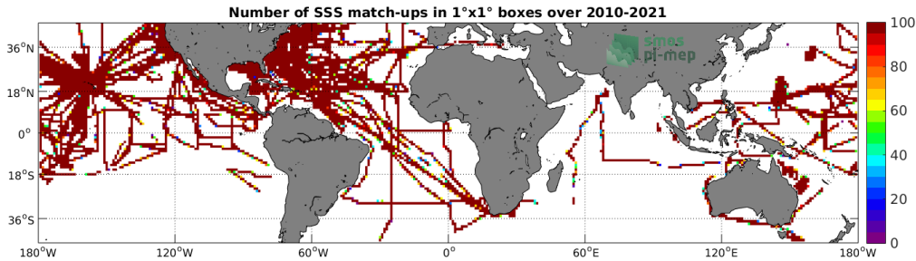
Figure 4: Number of SSS match-ups between TSG (SAMOS) SSS and the SMOS SSS L3 v317 - Monthly - 25 km (CATDS-CPDC) SSS product for the Mid-Low Latitudes 45N-45S Pi-MEP region over 1^\circ \times 1^\circ boxes and for the full satellite product period.
