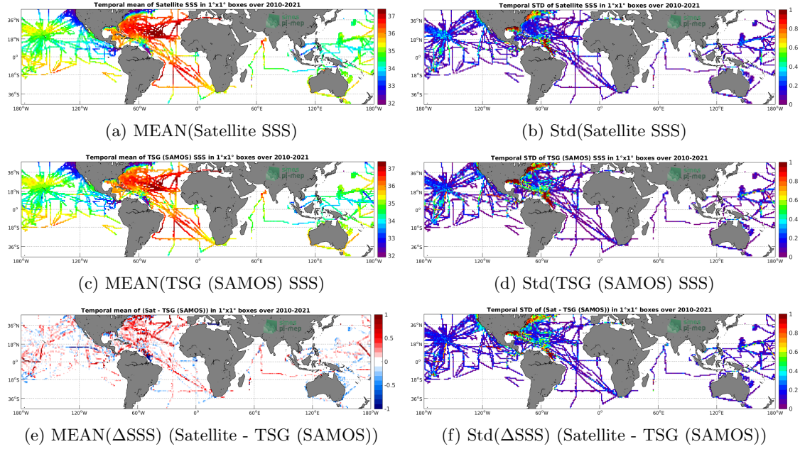
Figure 6: Temporal mean (left) and Std (right) of SSS from SMOS SSS L3 v317 - Monthly - 25 km (CATDS-CPDC) (top), TSG (SAMOS) (middle), and of \Delta SSS (Satellite - TSG (SAMOS)). Only match-up pairs are used to generate these maps.
