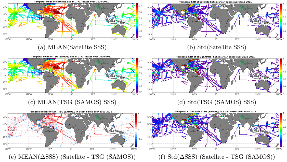
Figure 6: Temporal mean (left) and Std (right) of SSS from SMOS SSS L3 v317 - Monthly - 25 km (CATDS-CPDC) (top), TSG (SAMOS) (middle), and of \Delta SSS (Satellite - TSG (SAMOS)). Only match-up pairs are used to generate these maps.
