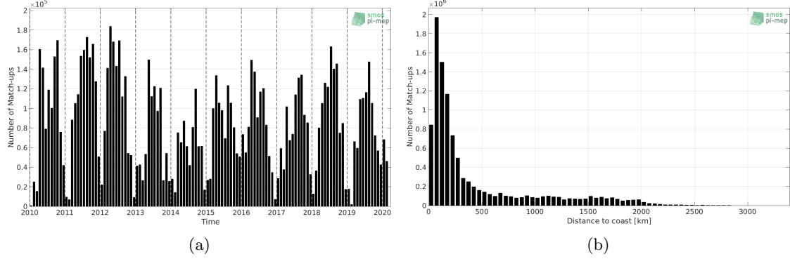
Figure 1: Number of match-ups between TSG-SAMOS and SMOS L3 v317 - Monthly - 25 km (CATDS-CPDC) SSS as a function of time (a) and as function of the distance to coast (b) over the Mid-Low Latitudes 45N-45S Pi-MEP region and for the full satellite product period.
