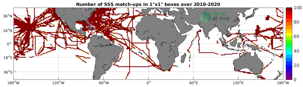
Figure 4: Number of SSS match-ups between TSG-SAMOS SSS and the SMOS L3 v317 - Monthly - 25 km (CATDS-CPDC) SSS product for the Mid-Low Latitudes 45N-45S Pi-MEP region over 1°x1° boxes and for the full satellite product period.
