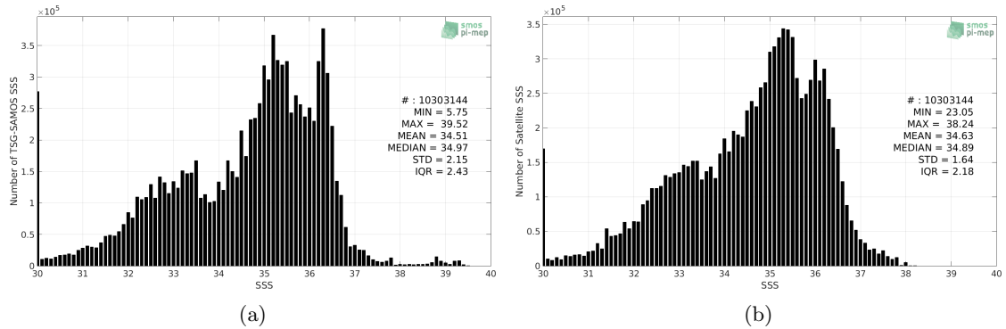
Figure 2: Histograms of SSS from TSG-SAMOS (a) and SMOS L3 v317 - Monthly - 25 km (CATDS-CPDC) (b) considering all match-up pairs per bins of 0.1 over the Mid-Low Latitudes 45N-45S Pi-MEP region and for the full satellite product period.
