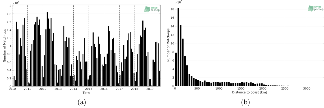
Figure 1: Number of match-ups between TSG-SAMOS and SMOS-L3-CATDS-CPDC-V317-MONTHLY-25KM SSS as a function of time (a) and as function of the distance to coast (b) over the Mid-Low Latitudes 45N-45S Pi-MEP region and for the full satellite product period.
