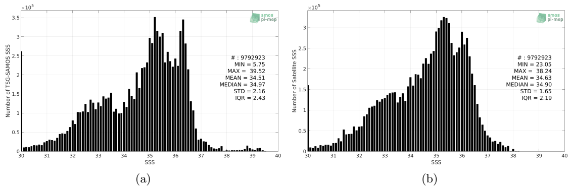
Figure 2: Histograms of SSS from TSG-SAMOS (a) and SMOS-L3-CATDS-CPDC-V317-MONTHLY-25KM (b) considering all match-up pairs per bins of 0.1 over the Mid-Low Latitudes 45N-45S Pi-MEP region and for the full satellite product period.
