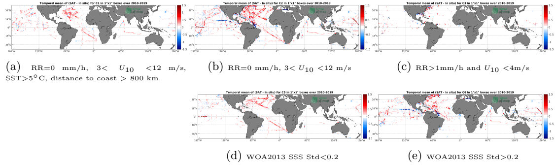
Figure 12: Temporal mean gridded over spatial boxes of size 1^\circ \times 1^\circ of \Delta SSS (SMOS-L3-CATDS-CPDC-V317-MONTHLY-25KM - TSG-SAMOS) for 5 different subdatasets corresponding to: RR=0 mm/h, 3 < U_{10} < 12 m/s, SST > 5^\circ\text{C} , distance to coast > 800 km (a), RR=0 mm/h, 3 < U_{10} < 12 m/s (b), RR > 1 mm/h and U_{10} < 4 m/s (c), WOA2013 SSS Std < 0.2 (d), WOA2013 SSS Std > 0.2 (e).
