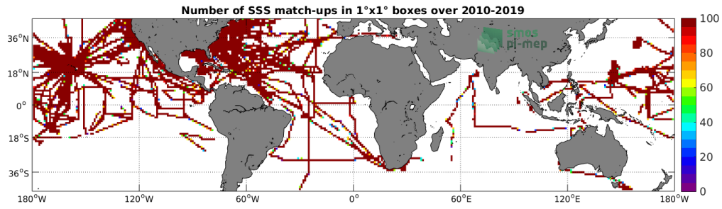
Figure 4: Number of SSS match-ups between TSG-SAMOS SSS and the SMOS-L3-CATDS-CPDC-V317-MONTHLY-25KM SSS product for the Mid-Low Latitudes 45N-45S Pi-MEP region over 1°x1° boxes and for the full satellite product period.
