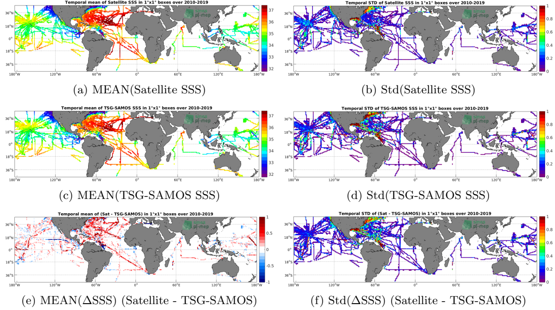
Figure 6: Temporal mean (left) and Std (right) of SSS from SMOS-L3-CATDS-CPDC-V317-MONTHLY-25KM (top), TSG-SAMOS (middle), and of \Delta SSS (Satellite - TSG-SAMOS). Only match-up pairs are used to generate these maps.
