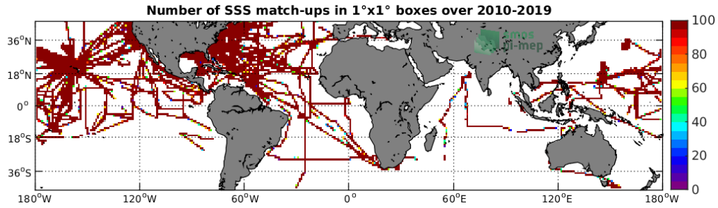
Figure 4: Number of SSS match-ups between TSG-SAMOS SSS and the SMOS-L3-CATDS-CPDC-V317-MONTHLY-25KM SSS product for the Mid-Low Latitudes 45N-45S Pi-MEP region over 1^\circ \times 1^\circ boxes and for the full satellite product period.
