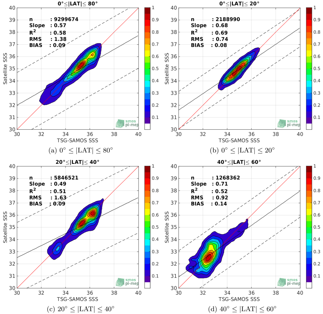
Figure 9: Contour maps of the concentration of SMOS-L3-CATDS-CPDC-V317-MONTHLY-25KM SSS (y-axis) versus TSG-SAMOS SSS (x-axis) at match-up pairs for different latitude bands. For each plot, the red line shows x=y . The black thin and dashed lines indicate a linear fit through the data cloud and the \pm 95\% confidence levels, respectively. The number match-up pairs n , the slope and R^2 coefficient of the linear fit, the root mean square (RMS) and the mean bias between satellite and in situ data are indicated for each latitude band in each plot.
