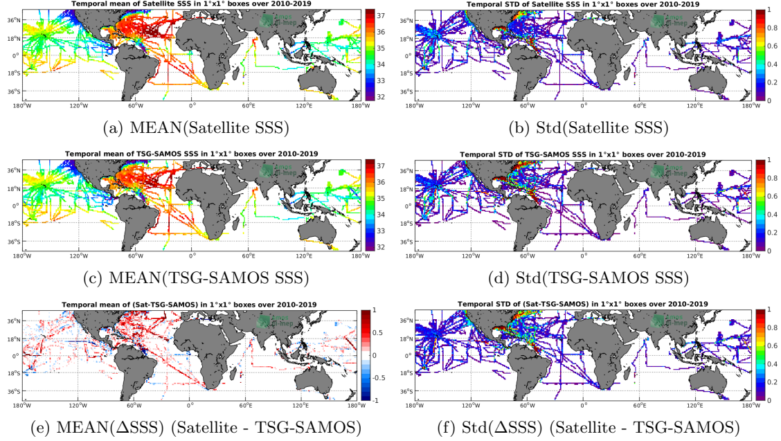
Figure 6: Temporal mean (left) and Std (right) of SSS from SMOS-L3-CATDS-CPDC-V317-MONTHLY-25KM (top), TSG-SAMOS (middle), and of \Delta SSS (Satellite - TSG-SAMOS). Only match-up pairs are used to generate these maps.
