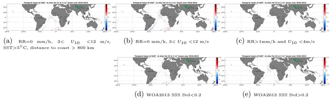
Figure 12: Temporal mean gridded over spatial boxes of size 1^\circ \times 1^\circ of \Delta SSS (SMOS SSS L3 v317 - Monthly - 25 km (CATDS-CPDC) - TSG (Polarstern)) for 5 different subdatasets corresponding to: RR=0 mm/h, 3 < U_{10} < 12 m/s, SST >5^\circ\text{C} , distance to coast > 800 km (a), RR=0 mm/h, 3 < U_{10} < 12 m/s (b), RR >1 mm/h and U_{10} < 4 m/s (c), WOA2013 SSS Std <0.2 (d), WOA2013 SSS Std >0.2 (e).
