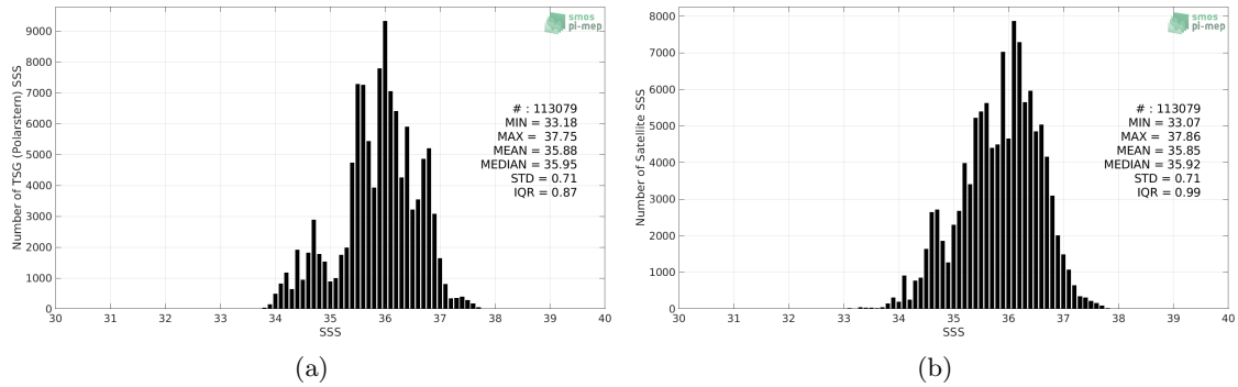
Figure 2: Histograms of SSS from TSG (Polarstern) (a) and SMOS SSS L3 v317 - Monthly - 25 km (CATDS-CPDC) (b) considering all match-up pairs per bins of 0.1 over the Mid-Low Latitudes 45N-45S Pi-MEP region and for the full satellite product period.
