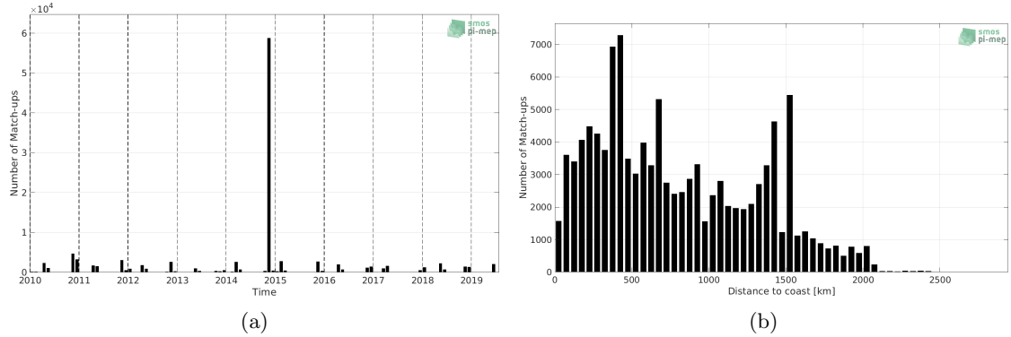
Figure 1: Number of match-ups between TSG (Polarstern) and SMOS SSS L3 v317 - Monthly - 25 km (CATDS-CPDC) SSS as a function of time (a) and as function of the distance to coast (b) over the Mid-Low Latitudes 45N-45S Pi-MEP region and for the full satellite product period.
