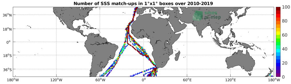
Figure 4: Number of SSS match-ups between TSG (Polarstern) SSS and the SMOS SSS L3 v317 - Monthly - 25 km (CATDS-CPDC) SSS product for the Mid-Low Latitudes 45N-45S Pi-MEP region over 1^\circ \times 1^\circ boxes and for the full satellite product period.
