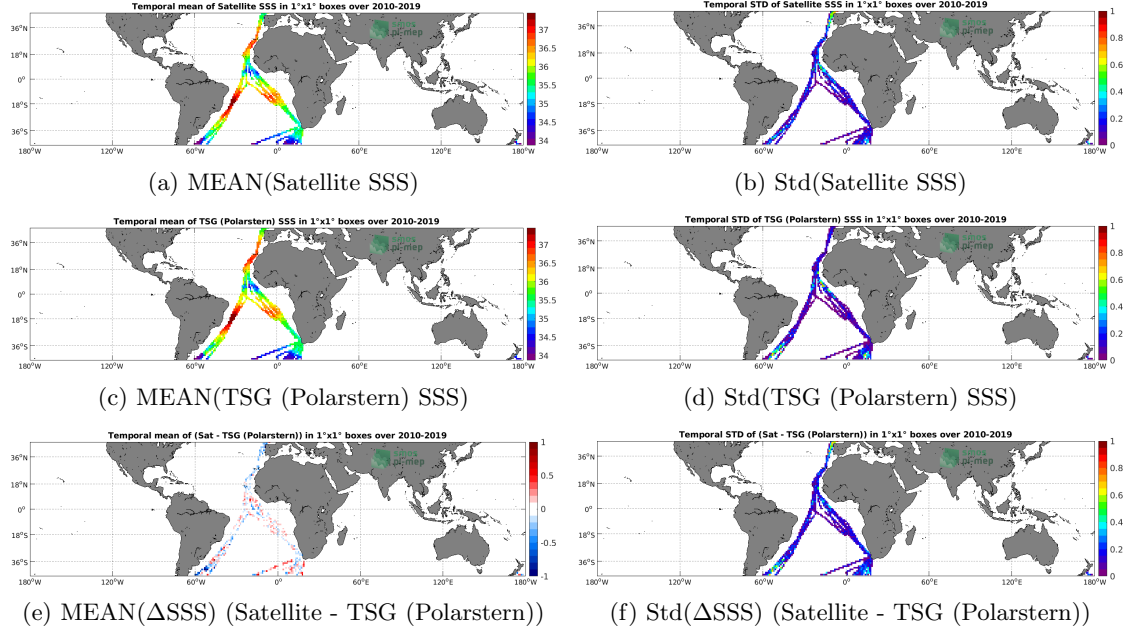
Figure 6: Temporal mean (left) and Std (right) of SSS from SMOS SSS L3 v317 - Monthly - 25 km (CATDS-CPDC) (top), TSG (Polarstern) (middle), and of \Delta SSS (Satellite - TSG (Polarstern)). Only match-up pairs are used to generate these maps.
