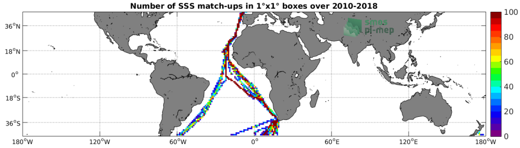
Figure 4: Number of SSS match-ups between TSG (Polarstern) SSS and the SMOS SSS L3 v317 - Monthly - 25 km (CATDS-CPDC) SSS product for the Mid-Low Latitudes 45N-45S Pi-MEP region over 1°x1° boxes and for the full satellite product period.
