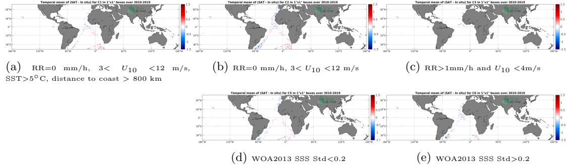
Figure 12: Temporal mean gridded over spatial boxes of size 1^\circ \times 1^\circ of \Delta SSS (SMOS L3 v317 - Monthly - 25 km (CATDS-CPDC) - TSG-POLARSTERN) for 5 different subdatasets corresponding to: RR=0 mm/h, 3 < U_{10} < 12 m/s, SST > 5^\circ C , distance to coast > 800 km (a), RR=0 mm/h, 3 < U_{10} < 12 m/s (b), RR > 1 mm/h and U_{10} < 4 m/s (c), WOA2013 SSS Std < 0.2 (d), WOA2013 SSS Std > 0.2 (e).
