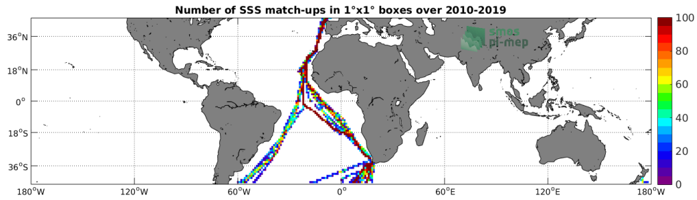
Figure 4: Number of SSS match-ups between TSG-POLARSTERN SSS and the SMOS L3 v317 - Monthly - 25 km (CATDS-CPDC) SSS product for the Mid-Low Latitudes 45N-45S Pi-MEP region over 1°x1° boxes and for the full satellite product period.
