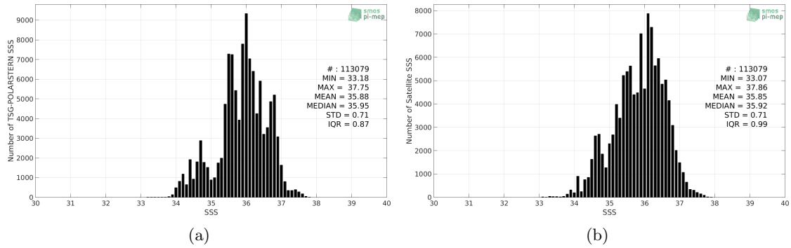
Figure 2: Histograms of SSS from TSG-POLARSTERN (a) and SMOS L3 v317 - Monthly - 25 km (CATDS-CPDC) (b) considering all match-up pairs per bins of 0.1 over the Mid-Low Latitudes 45N-45S Pi-MEP region and for the full satellite product period.
