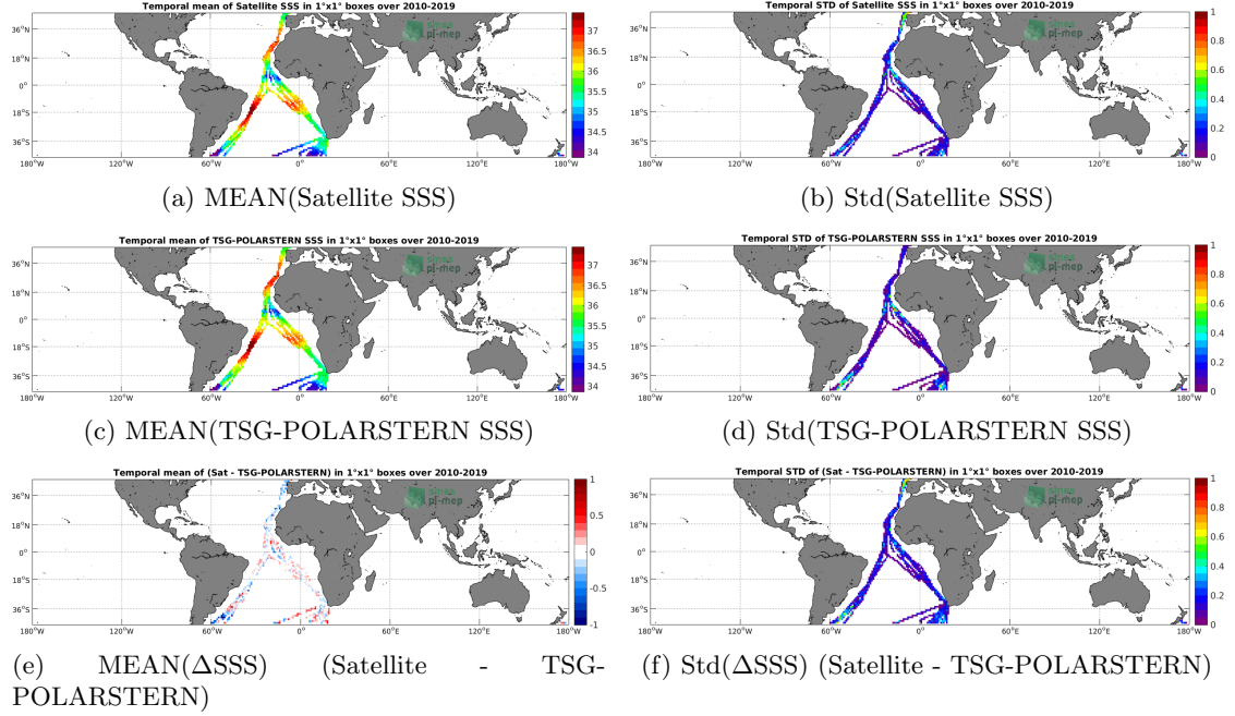
Figure 6: Temporal mean (left) and Std (right) of SSS from SMOS L3 v317 - Monthly - 25 km (CATDS-CPDC) (top), TSG-POLARSTERN (middle), and of \Delta SSS (Satellite - TSG-POLARSTERN). Only match-up pairs are used to generate these maps.
