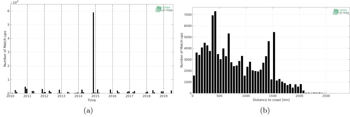
Figure 1: Number of match-ups between TSG-POLARSTERN and SMOS L3 v317 - Monthly - 25 km (CATDS-CPDC) SSS as a function of time (a) and as function of the distance to coast (b) over the Mid-Low Latitudes 45N-45S Pi-MEP region and for the full satellite product period.
