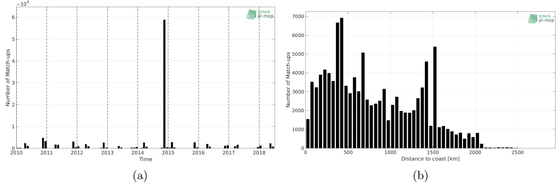
Figure 1: Number of match-ups between TSG-POLARSTERN and SMOS-L3-CATDS-CPDC-V317-MONTHLY-25KM SSS as a function of time (a) and as function of the distance to coast (b) over the Mid-Low Latitudes 45N-45S Pi-MEP region and for the full satellite product period.
