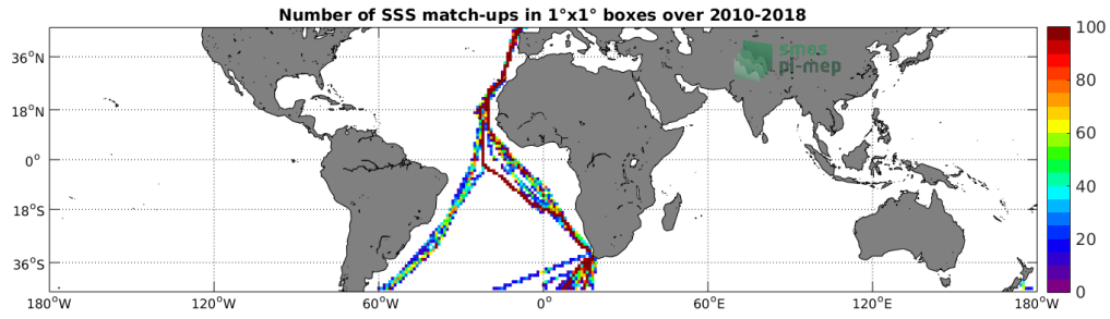
Figure 4: Number of SSS match-ups between TSG-POLARSTERN SSS and the SMOS-L3-CATDS-CPDC-V317-MONTHLY-25KM SSS product for the Mid-Low Latitudes 45N-45S Pi-MEP region over 1^\circ \times 1^\circ boxes and for the full satellite product period.
