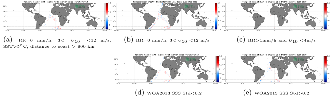
Figure 12: Temporal mean gridded over spatial boxes of size 1^\circ \times 1^\circ of \Delta SSS (SMOS-L3-CATDS-CPDC-V317-MONTHLY-25KM - TSG-POLARSTERN) for 5 different subdatasets corresponding to: RR=0 mm/h, 3 < U_{10} < 12 m/s, SST > 5^\circ C , distance to coast > 800 km (a), RR=0 mm/h, 3 < U_{10} < 12 m/s (b), RR > 1 mm/h and U_{10} < 4 m/s (c), WOA2013 SSS Std < 0.2 (d), WOA2013 SSS Std > 0.2 (e).
