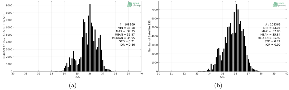
Figure 2: Histograms of SSS from TSG-POLARSTERN (a) and SMOS-L3-CATDS-CPDC-V317-MONTHLY-25KM (b) considering all match-up pairs per bins of 0.1 over the Mid-Low Latitudes 45N-45S Pi-MEP region and for the full satellite product period.
