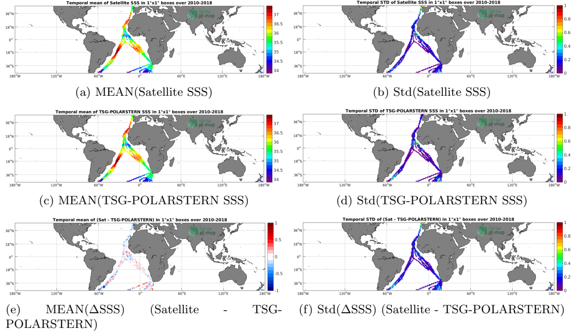
Figure 6: Temporal mean (left) and Std (right) of SSS from SMOS-L3-CATDS-CPDC-V317-MONTHLY-25KM (top), TSG-POLARSTERN (middle), and of \Delta SSS (Satellite - TSG-POLARSTERN). Only match-up pairs are used to generate these maps.
