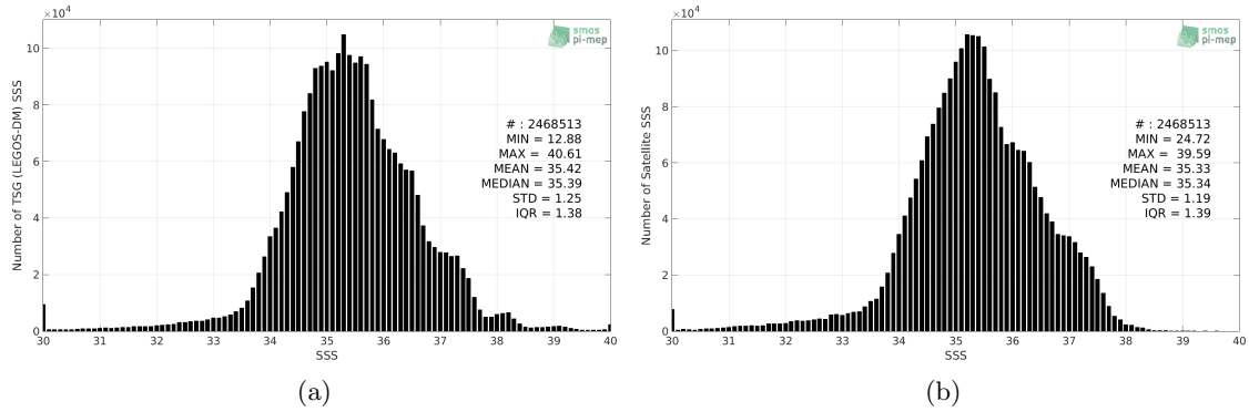
Figure 2: Histograms of SSS from TSG (LEGOS-DM) (a) and SMOS SSS L3 v317 - Monthly - 25 km (CATDS-CPDC) (b) considering all match-up pairs per bins of 0.1 over the Mid-Low Latitudes 45N-45S Pi-MEP region and for the full satellite product period.
