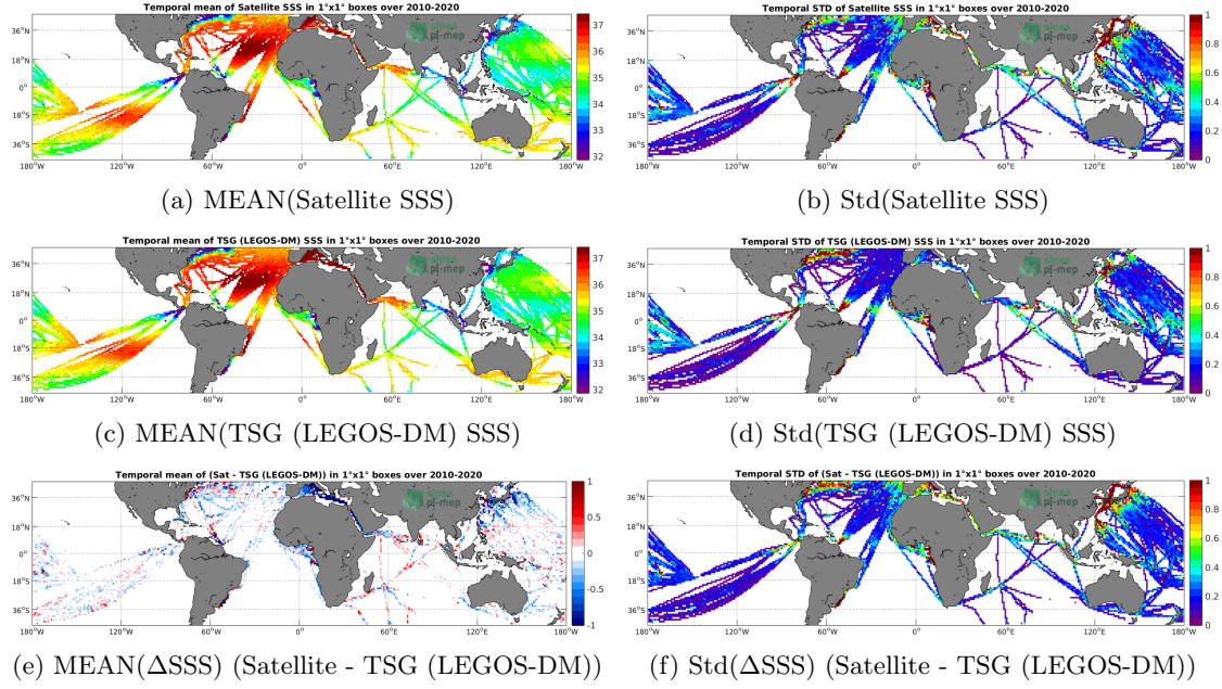
Figure 6: Temporal mean (left) and Std (right) of SSS from SMOS SSS L3 v317 - Monthly - 25 km (CATDS-CPDC) (top), TSG (LEGOS-DM) (middle), and of \Delta SSS (Satellite - TSG (LEGOS-DM)). Only match-up pairs are used to generate these maps.
