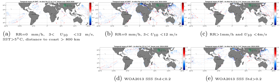
Figure 12: Temporal mean gridded over spatial boxes of size 1^\circ \times 1^\circ of \Delta SSS (SMOS SSS L3 v317 - Monthly - 25 km (CATDS-CPDC) - TSG (LEGOS-DM)) for 5 different subdatasets corresponding to: RR=0 mm/h, 3 < U_{10} < 12 m/s, SST > 5^\circ C , distance to coast > 800 km (a), RR=0 mm/h, 3 < U_{10} < 12 m/s (b), RR > 1 mm/h and U_{10} < 4 m/s (c), WOA2013 SSS Std < 0.2 (d), WOA2013 SSS Std > 0.2 (e).
