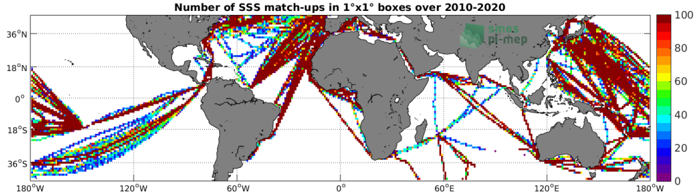
Figure 4: Number of SSS match-ups between TSG (LEGOS-DM) SSS and the SMOS SSS L3 v317 - Monthly - 25 km (CATDS-CPDC) SSS product for the Mid-Low Latitudes 45N-45S Pi-MEP region over 1^\circ \times 1^\circ boxes and for the full satellite product period.
