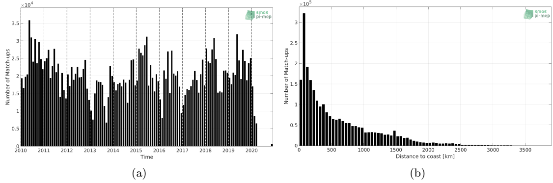
Figure 1: Number of match-ups between TSG (LEGOS-DM) and SMOS SSS L3 v317 - Monthly - 25 km (CATDS-CPDC) SSS as a function of time (a) and as function of the distance to coast (b) over the Mid-Low Latitudes 45N-45S Pi-MEP region and for the full satellite product period.
