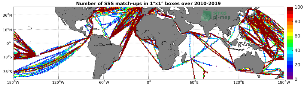
Figure 4: Number of SSS match-ups between TSG (LEGOS-DM) SSS and the SMOS SSS L3 v317 - Monthly - 25 km (CATDS-CPDC) SSS product for the Mid-Low Latitudes 45N-45S Pi-MEP region over 1°x1° boxes and for the full satellite product period.
