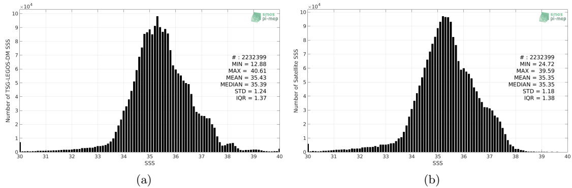
Figure 2: Histograms of SSS from TSG-LEGOS-DM (a) and SMOS L3 v317 - Monthly - 25 km (CATDS-CPDC) (b) considering all match-up pairs per bins of 0.1 over the Mid-Low Latitudes 45N-45S Pi-MEP region and for the full satellite product period.
