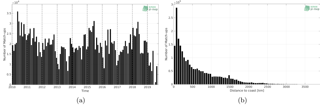
Figure 1: Number of match-ups between TSG-LEGOS-DM and SMOS L3 v317 - Monthly - 25 km (CATDS-CPDC) SSS as a function of time (a) and as function of the distance to coast (b) over the Mid-Low Latitudes 45N-45S Pi-MEP region and for the full satellite product period.
