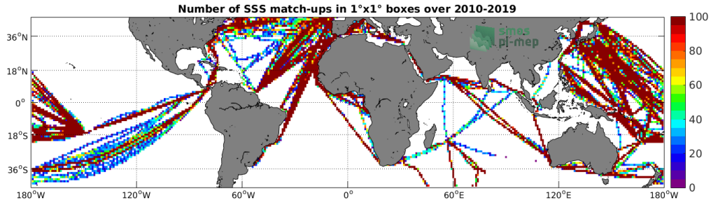
Figure 4: Number of SSS match-ups between TSG-LEGOS-DM SSS and the SMOS L3 v317 - Monthly - 25 km (CATDS-CPDC) SSS product for the Mid-Low Latitudes 45N-45S Pi-MEP region over 1°x1° boxes and for the full satellite product period.
