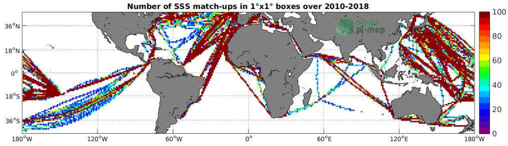
Figure 4: Number of SSS match-ups between TSG-LEGOS-DM SSS and the SMOS-L3-CATDS-CPDC-V317-MONTHLY-25KM SSS product for the Mid-Low Latitudes 45N-45S Pi-MEP region over 1°x1° boxes and for the full satellite product period.
