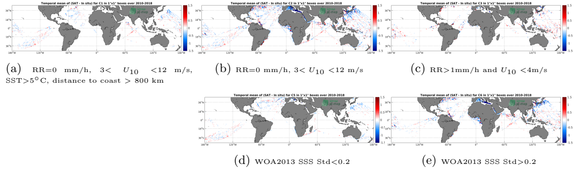
Figure 12: Temporal mean gridded over spatial boxes of size 1^\circ \times 1^\circ of \Delta SSS (SMOS-L3-CATDS-CPDC-V317-MONTHLY-25KM - TSG-LEGOS-DM) for 5 different subdatasets corresponding to: RR=0 mm/h, 3 < U_{10} < 12 m/s, SST > 5^\circ C , distance to coast > 800 km (a), RR=0 mm/h, 3 < U_{10} < 12 m/s (b), RR > 1 mm/h and U_{10} < 4 m/s (c), WOA2013 SSS Std < 0.2 (d), WOA2013 SSS Std > 0.2 (e).
