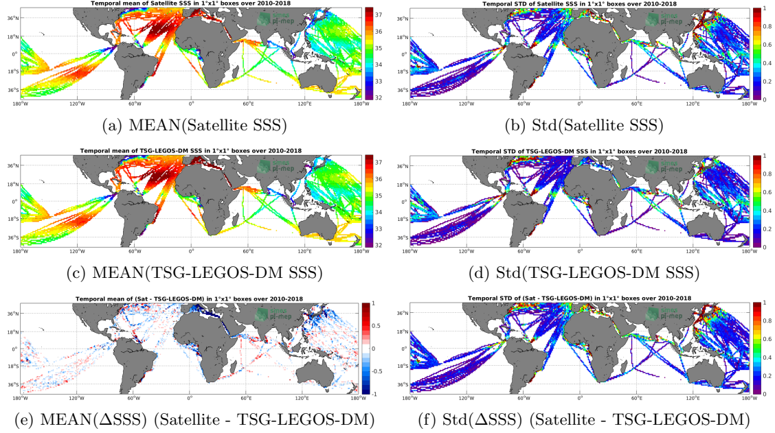
Figure 6: Temporal mean (left) and Std (right) of SSS from SMOS-L3-CATDS-CPDC-V317-MONTHLY-25KM satellite SSS product (in black), TSG-LEGOS-DM (middle), and of \Delta SSS (Satellite - TSG-LEGOS-DM). Only match-up pairs are used to generate these maps.
