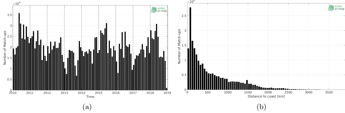
Figure 1: Number of match-ups between TSG-LEGOS-DM and SMOS-L3-CATDS-CPDC-V317-MONTHLY-25KM SSS as a function of time (a) and as function of the distance to coast (b) over the Mid-Low Latitudes 45N-45S Pi-MEP region and for the full satellite product period.
