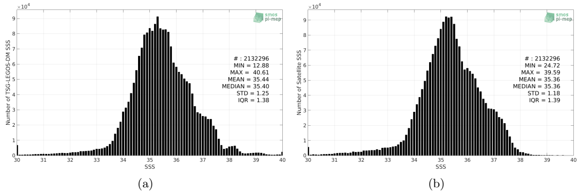
Figure 2: Histograms of SSS from TSG-LEGOS-DM (a) and SMOS-L3-CATDS-CPDC-V317-MONTHLY-25KM (b) considering all match-up pairs per bins of 0.1 over the Mid-Low Latitudes 45N-45S Pi-MEP region and for the full satellite product period.
