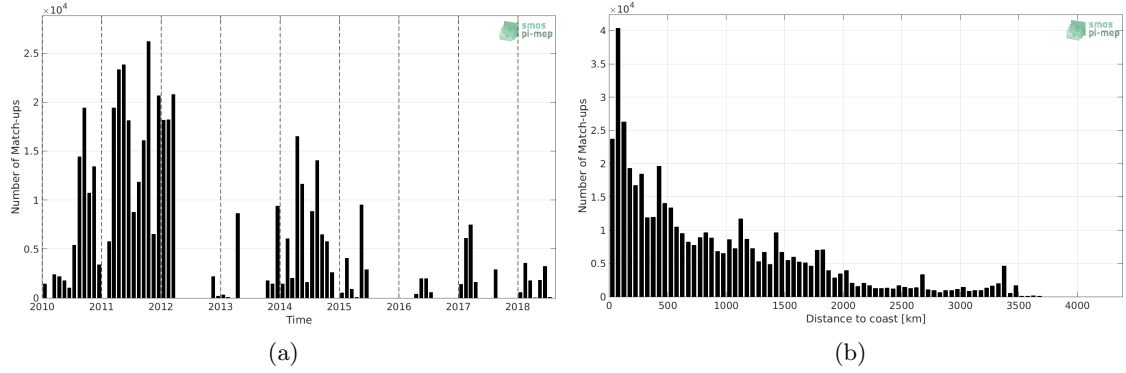
Figure 1: Number of match-ups between TSG (GOSUD-Sailing-ship) and SMOS SSS L3 v317 - Monthly - 25 km (CATDS-CPDC) SSS as a function of time (a) and as function of the distance to coast (b) over the Mid-Low Latitudes 45N-45S Pi-MEP region and for the full satellite product period.
