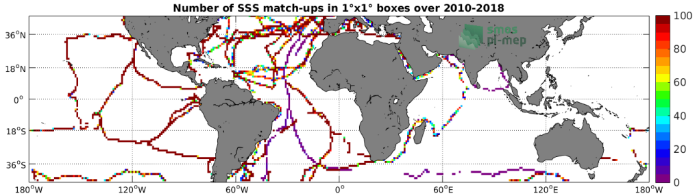
Figure 4: Number of SSS match-ups between TSG (GOSUD-Sailing-ship) SSS and the SMOS SSS L3 v317 - Monthly - 25 km (CATDS-CPDC) SSS product for the Mid-Low Latitudes 45N-45S Pi-MEP region over 1^\circ \times 1^\circ boxes and for the full satellite product period.
