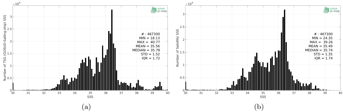
Figure 2: Histograms of SSS from TSG (GOSUD-Sailing-ship) (a) and SMOS SSS L3 v317 - Monthly - 25 km (CATDS-CPDC) (b) considering all match-up pairs per bins of 0.1 over the Mid-Low Latitudes 45N-45S Pi-MEP region and for the full satellite product period.
