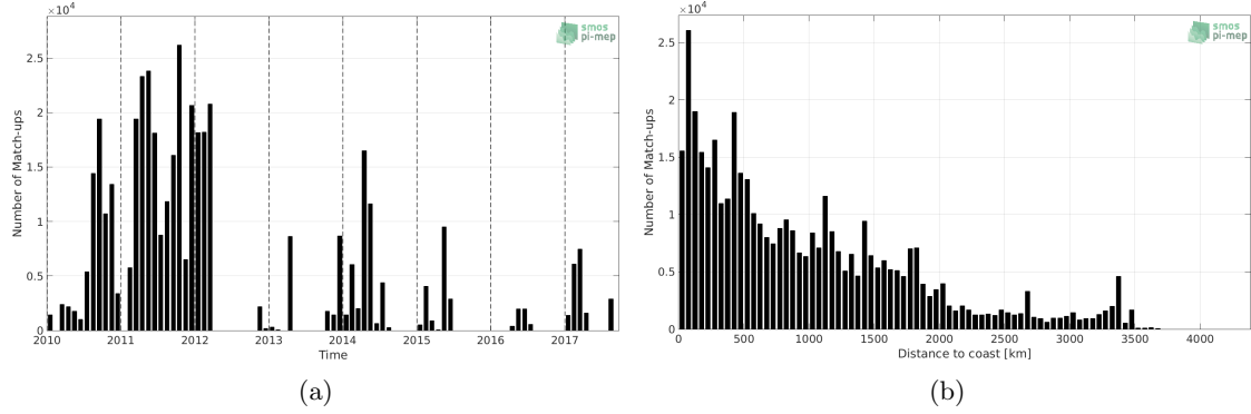
Figure 1: Number of match-ups between TSG-GOSUD-Sailing-ship and SMOS L3 v317 - Monthly - 25 km (CATDS-CPDC) SSS as a function of time (a) and as function of the distance to coast (b) over the Mid-Low Latitudes 45N-45S Pi-MEP region and for the full satellite product period.
