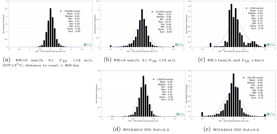
Figure 13: Normalized histogram of \Delta\text{SSS} (SMOS L3 v317 - Monthly - 25 km (CATDS-CPDC) - TSG-GOSUD-Sailing-ship) for 5 different subdatasets corresponding to: RR=0 mm/h, 3 < U_{10} < 12 m/s, SST > 5^\circ\text{C} , distance to coast > 800 km (a), RR=0 mm/h, 3 < U_{10} < 12 m/s (b), RR > 1\text{mm/h} and U_{10} < 4\text{m/s} (c), WOA2013 SSS Std < 0.2 (d), WOA2013 SSS Std > 0.2 (e).
