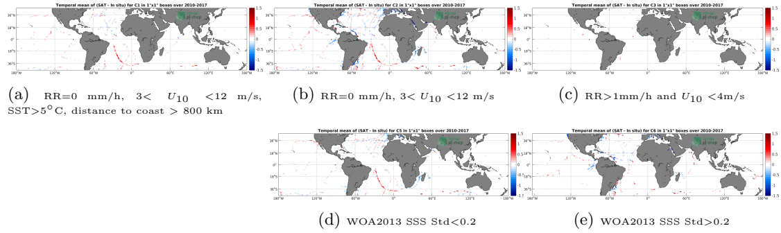
Figure 12: Temporal mean gridded over spatial boxes of size 1^\circ \times 1^\circ of \Delta SSS (SMOS L3 v317 - Monthly - 25 km (CATDS-CPDC) - TSG-GOSUD-Sailing-ship) for 5 different subdatasets corresponding to: RR=0 mm/h, 3 < U_{10} < 12 m/s, SST > 5^\circ C , distance to coast > 800 km (a), RR=0 mm/h, 3 < U_{10} < 12 m/s (b), RR > 1 mm/h and U_{10} < 4 m/s (c), WOA2013 SSS Std < 0.2 (d), WOA2013 SSS Std > 0.2 (e).
