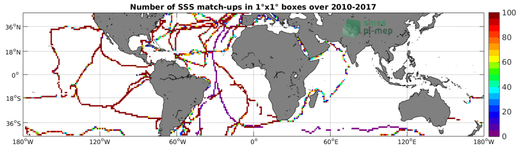
Figure 4: Number of SSS match-ups between TSG-GOSUD-Sailing-ship SSS and the SMOS L3 v317 - Monthly - 25 km (CATDS-CPDC) SSS product for the Mid-Low Latitudes 45N-45S Pi-MEP region over 1°x1° boxes and for the full satellite product period.
