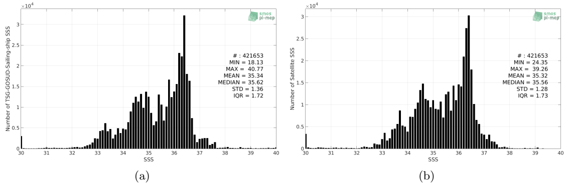
Figure 2: Histograms of SSS from TSG-GOSUD-Sailing-ship (a) and SMOS L3 v317 - Monthly - 25 km (CATDS-CPDC) (b) considering all match-up pairs per bins of 0.1 over the Mid-Low Latitudes 45N-45S Pi-MEP region and for the full satellite product period.
