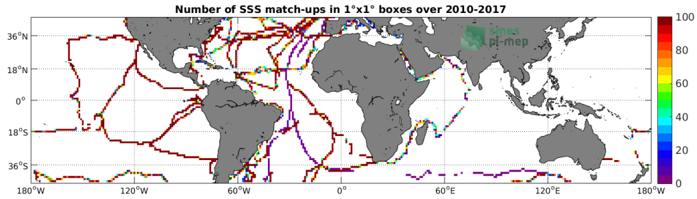
Figure 4: Number of SSS match-ups between TSG-GOSUD-Sailing-ship SSS and the SMOS-L3-CATDS-CPDC-V317-MONTHLY-25KM SSS product for the Mid-Low Latitudes 45N-45S Pi-MEP region over 1°x1° boxes and for the full satellite product period.
