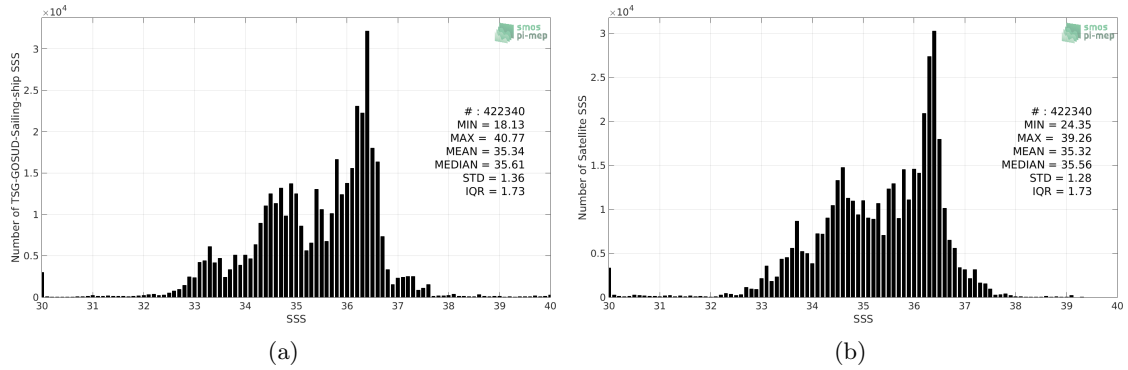
Figure 2: Histograms of SSS from TSG-GOSUD-Sailing-ship (a) and SMOS-L3-CATDS-CPDC-V317-MONTHLY-25KM (b) considering all match-up pairs per bins of 0.1 over the Mid-Low Latitudes 45N-45S Pi-MEP region and for the full satellite product period.
