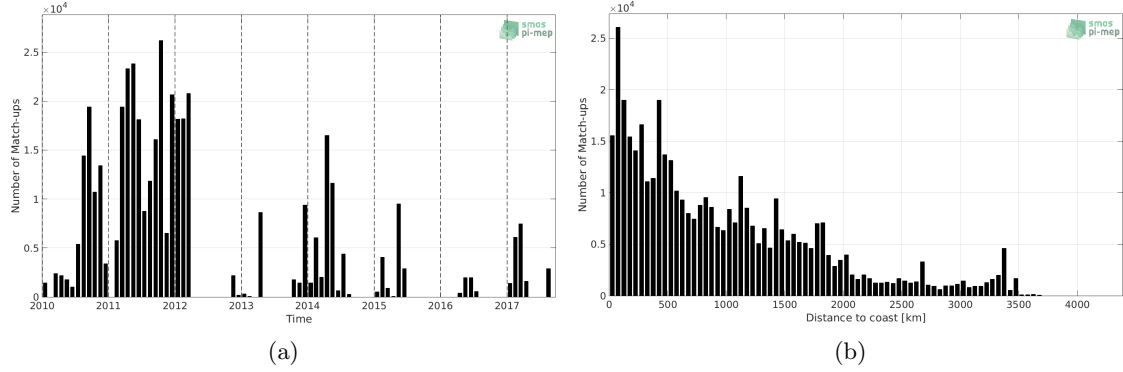
Figure 1: Number of match-ups between TSG-GOSUD-Sailing-ship and SMOS-L3-CATDS-CPDC-V317-MONTHLY-25KM SSS as a function of time (a) and as function of the distance to coast (b) over the Mid-Low Latitudes 45N-45S Pi-MEP region and for the full satellite product period.
