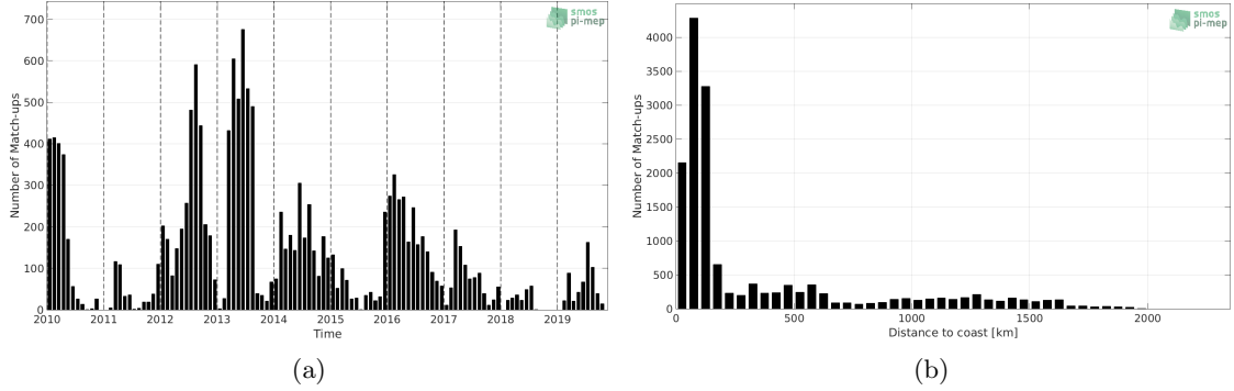
Figure 1: Number of match-ups between Marine mammals and SMOS SSS L3 v317 - Monthly - 25 km (CATDS-CPDC) SSS as a function of time (a) and as function of the distance to coast (b) over the Mid-Low Latitudes 45N-45S Pi-MEP region and for the full satellite product period.
