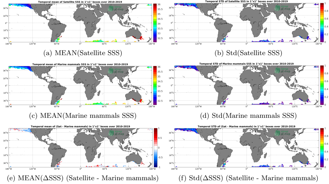
Figure 6: Temporal mean (left) and Std (right) of SSS from SMOS SSS L3 v317 - Monthly - 25 km (CATDS-CPDC) (top), Marine mammals (middle), and of \Delta SSS (Satellite - Marine mammals). Only match-up pairs are used to generate these maps.
