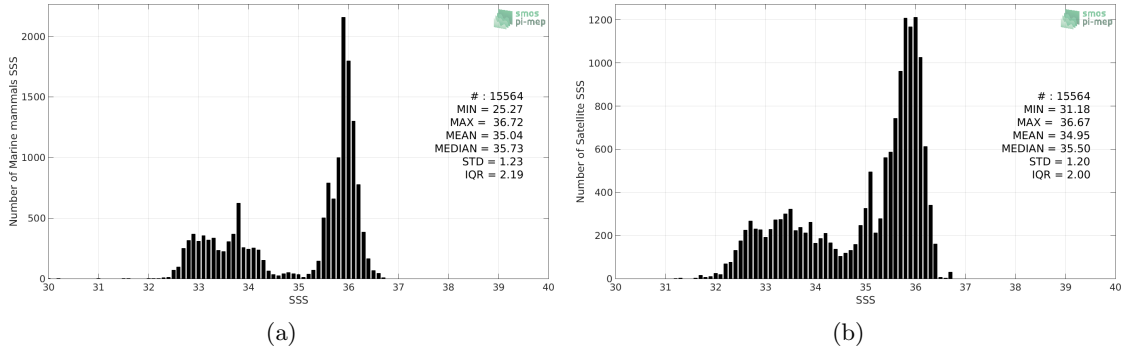
Figure 2: Histograms of SSS from Marine mammals (a) and SMOS SSS L3 v317 - Monthly - 25 km (CATDS-CPDC) (b) considering all match-up pairs per bins of 0.1 over the Mid-Low Latitudes 45N-45S Pi-MEP region and for the full satellite product period.
