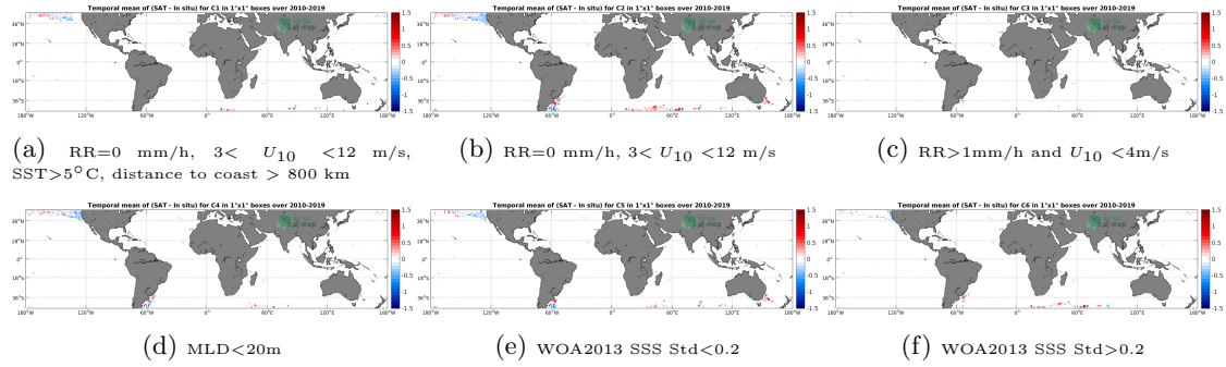
Figure 12: Temporal mean gridded over spatial boxes of size 1^\circ \times 1^\circ of \Delta SSS (SMOS SSS L3 v317 - Monthly - 25 km (CATDS-CPDC) - Marine mammals) for 6 different subdatasets corresponding to: RR=0 mm/h, 3 < U_{10} < 12 m/s, SST > 5^\circ C , distance to coast > 800 km (a), RR=0 mm/h, 3 < U_{10} < 12 m/s (b), RR > 1 mm/h and U_{10} < 4 m/s (c), MLD < 20 m (d), WOA2013 SSS Std < 0.2 (e), WOA2013 SSS Std > 0.2 (f).
