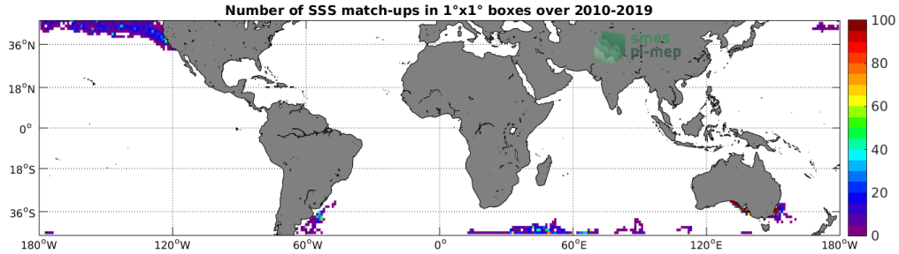
Figure 4: Number of SSS match-ups between Marine mammals SSS and the SMOS SSS L3 v317 - Monthly - 25 km (CATDS-CPDC) SSS product for the Mid-Low Latitudes 45N-45S Pi-MEP region over 1^\circ \times 1^\circ boxes and for the full satellite product period.
