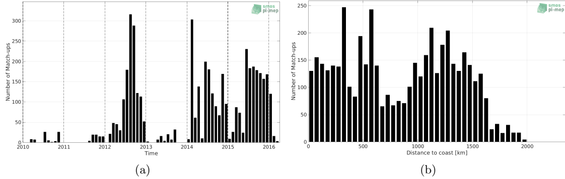
Figure 1: Number of match-ups between Sea mammals and SMOS SSS L3 v317 - Monthly - 25 km (CATDS-CPDC) SSS as a function of time (a) and as function of the distance to coast (b) over the Mid-Low Latitudes 45N-45S Pi-MEP region and for the full satellite product period.
