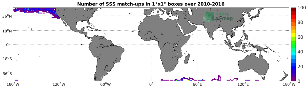
Figure 4: Number of SSS match-ups between Sea mammals SSS and the SMOS SSS L3 v317 - Monthly - 25 km (CATDS-CPDC) SSS product for the Mid-Low Latitudes 45N-45S Pi-MEP region over 1^\circ \times 1^\circ boxes and for the full satellite product period.
