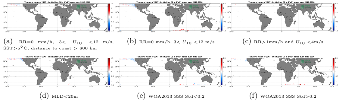
Figure 12: Temporal mean gridded over spatial boxes of size 1^\circ \times 1^\circ of \Delta SSS (SMOS SSS L3 v317 - Monthly - 25 km (CATDS-CPDC) - Sea mammals) for 6 different subdatasets corresponding to: RR=0 mm/h, 3 < U_{10} < 12 m/s, SST > 5^\circ C , distance to coast > 800 km (a), RR=0 mm/h, 3 < U_{10} < 12 m/s (b), RR > 1 mm/h and U_{10} < 4 m/s (c), MLD < 20 m (d), WOA2013 SSS Std < 0.2 (e), WOA2013 SSS Std > 0.2 (f).
