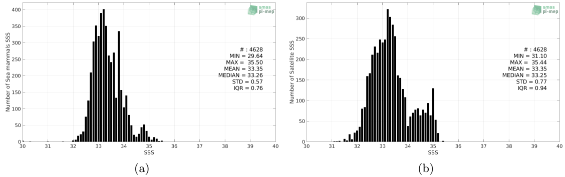
Figure 2: Histograms of SSS from Sea mammals (a) and SMOS SSS L3 v317 - Monthly - 25 km (CATDS-CPDC) (b) considering all match-up pairs per bins of 0.1 over the Mid-Low Latitudes 45N-45S Pi-MEP region and for the full satellite product period.
