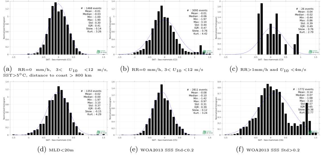
Figure 13: Normalized histogram of \Delta SSS (SMOS SSS L3 v317 - Monthly - 25 km (CATDS-CPDC) - Sea mammals) for 6 different subdatasets corresponding to: RR=0 mm/h, 3 < U_{10} < 12 m/s, SST>5°C, distance to coast > 800 km (a), RR=0 mm/h, 3 < U_{10} < 12 m/s (b), RR>1mm/h and U_{10} < 4 m/s (c), MLD<20m (d), WOA2013 SSS Std<0.2 (e), WOA2013 SSS Std>0.2 (f).
