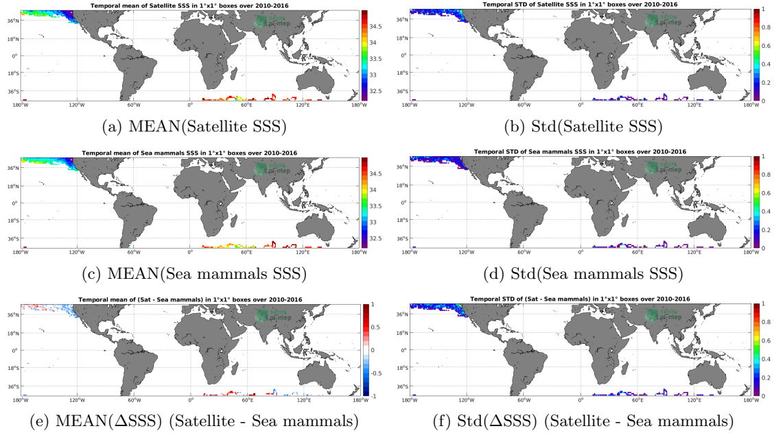
Figure 6: Temporal mean (left) and Std (right) of SSS from SMOS SSS L3 v317 - Monthly - 25 km (CATDS-CPDC) (top), Sea mammals (middle), and of \Delta SSS (Satellite - Sea mammals). Only match-up pairs are used to generate these maps.
