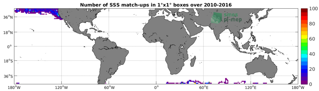
Figure 4: Number of SSS match-ups between Sea mammals SSS and the SMOS SSS L3 v317 - Monthly - 25 km (CATDS-CPDC) SSS product for the Mid-Low Latitudes 45N-45S Pi-MEP region over 1°x1° boxes and for the full satellite product period.
