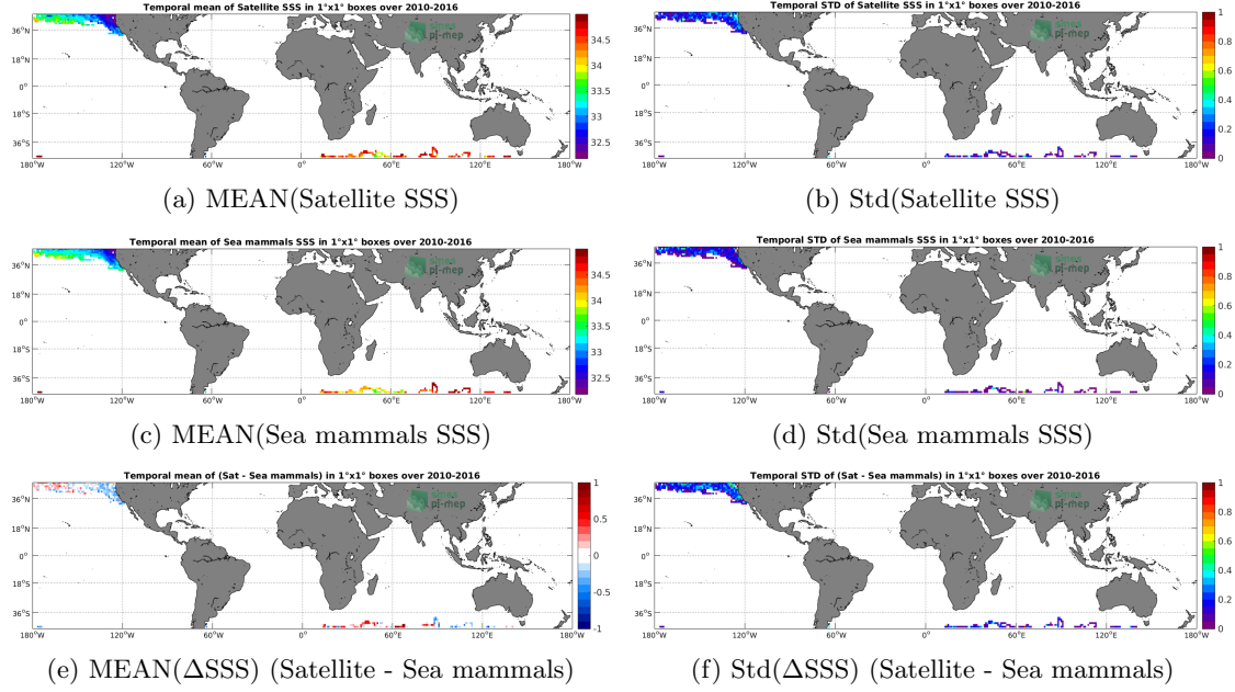
Figure 6: Temporal mean (left) and Std (right) of SSS from SMOS SSS L3 v317 - Monthly - 25 km (CATDS-CPDC) (top), Sea mammals (middle), and of \Delta SSS (Satellite - Sea mammals). Only match-up pairs are used to generate these maps.
