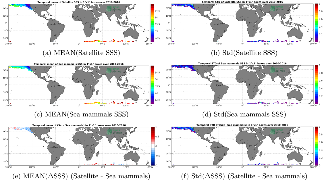
Figure 6: Temporal mean (left) and Std (right) of SSS from SMOS L3 v317 - Monthly - 25 km (CATDS-CPDC) (top), Sea mammals (middle), and of \Delta SSS (Satellite - Sea mammals). Only match-up pairs are used to generate these maps.
