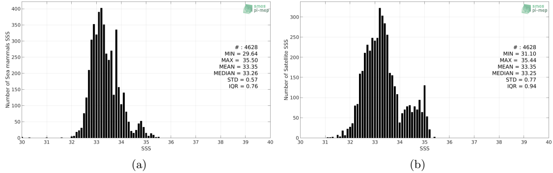
Figure 2: Histograms of SSS from Sea mammals (a) and SMOS L3 v317 - Monthly - 25 km (CATDS-CPDC) (b) considering all match-up pairs per bins of 0.1 over the Mid-Low Latitudes 45N-45S Pi-MEP region and for the full satellite product period.
