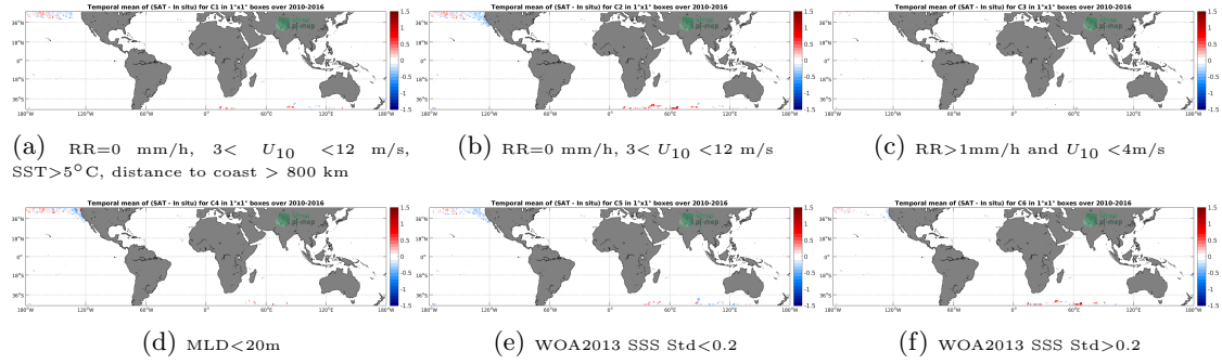
Figure 12: Temporal mean gridded over spatial boxes of size 1^\circ \times 1^\circ of \Delta SSS (SMOS L3 v317 - Monthly - 25 km (CATDS-CPDC) - Sea mammals) for 6 different subdatasets corresponding to: RR=0 mm/h, 3 < U_{10} < 12 m/s, SST >5^\circ\text{C} , distance to coast > 800 km (a), RR=0 mm/h, 3 < U_{10} < 12 m/s (b), RR >1 mm/h and U_{10} < 4 m/s (c),MLD <20 m (d),WOA2013 SSS Std <0.2 (e),WOA2013 SSS Std >0.2 (f).
