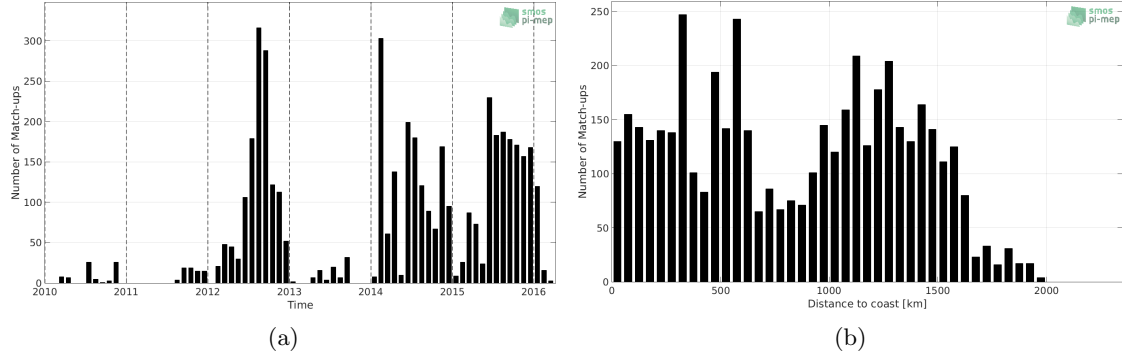
Figure 1: Number of match-ups between Sea mammals and SMOS L3 v317 - Monthly - 25 km (CATDS-CPDC) SSS as a function of time (a) and as function of the distance to coast (b) over the Mid-Low Latitudes 45N-45S Pi-MEP region and for the full satellite product period.
