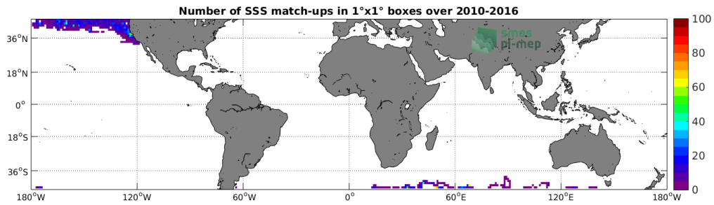
Figure 4: Number of SSS match-ups between Sea mammals SSS and the SMOS L3 v317 - Monthly - 25 km (CATDS-CPDC) SSS product for the Mid-Low Latitudes 45N-45S Pi-MEP region over 1°x1° boxes and for the full satellite product period.
