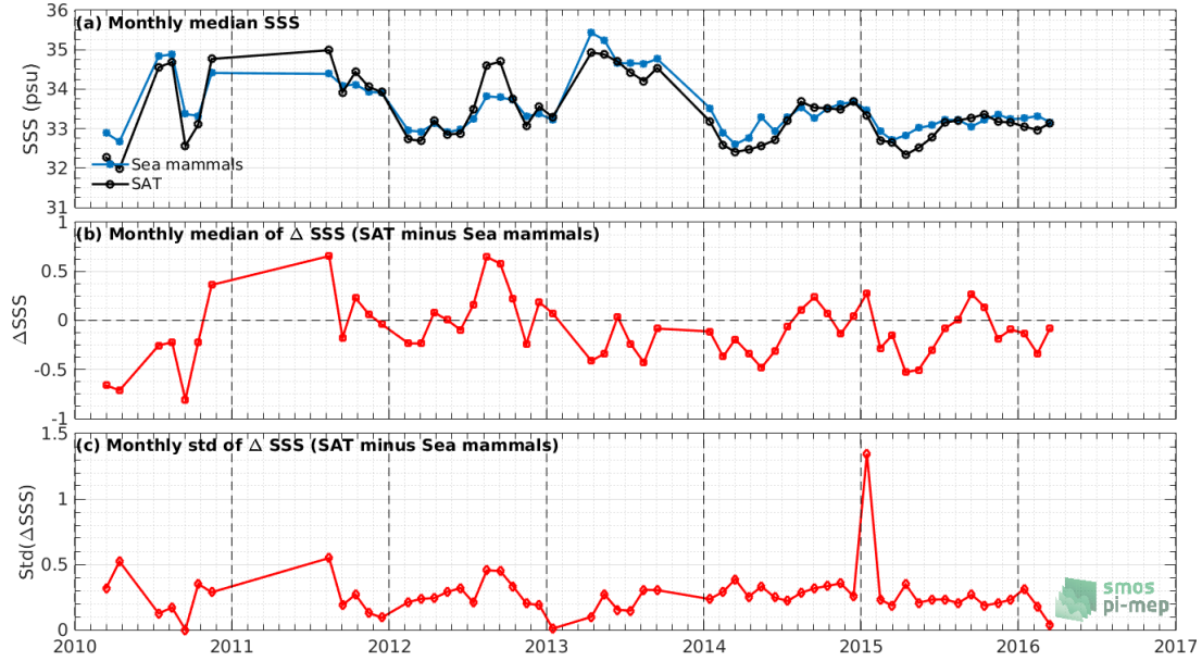
Figure 7: Time series of the monthly median SSS (top), median of \Delta\text{SSS} (Satellite - Sea mammals) and Std of \Delta\text{SSS} (Satellite - Sea mammals) over the Mid-Low Latitudes 45N-45S Pi-MEP region considering all match-ups collected by the Pi-MEP.
