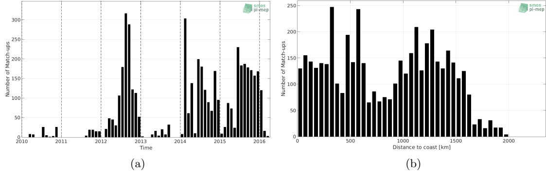
Figure 1: Number of match-ups between Sea mammals and SMOS-L3-CATDS-CPDC-V317-MONTHLY-25KM SSS as a function of time (a) and as function of the distance to coast (b) over the Mid-Low Latitudes 45N-45S Pi-MEP region and for the full satellite product period.
