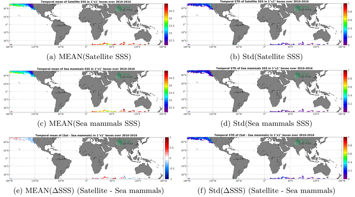
Figure 6: Temporal mean (left) and Std (right) of SSS from SMOS-L3-CATDS-CPDC-V317-MONTHLY-25KM (top), Sea mammals (middle), and of \Delta SSS (Satellite - Sea mammals). Only match-up pairs are used to generate these maps.
