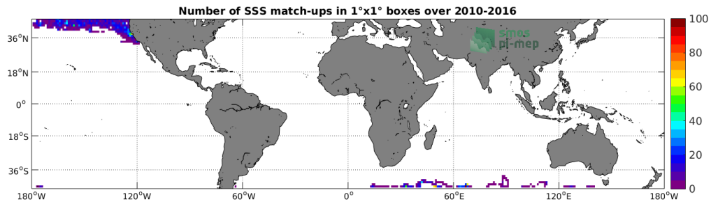
Figure 4: Number of SSS match-ups between Sea mammals SSS and the SMOS-L3-CATDS-CPDC-V317-MONTHLY-25KM SSS product for the Mid-Low Latitudes 45N-45S Pi-MEP region over 1°x1° boxes and for the full satellite product period.
