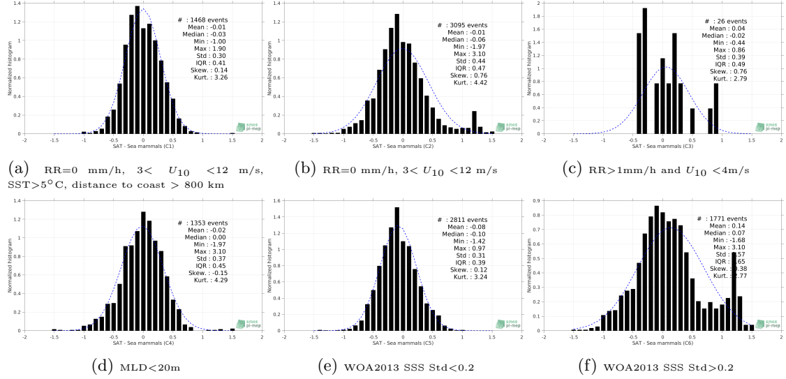
Figure 13: Normalized histogram of \Delta SSS (SMOS-L3-CATDS-CPDC-V317-MONTHLY-25KM - Sea mammals) for 6 different subdatasets corresponding to: RR=0 mm/h, 3 < U_{10} < 12 m/s, SST > 5^\circ C , distance to coast > 800 km (a), RR=0 mm/h, 3 < U_{10} < 12 m/s (b), RR > 1 mm/h and U_{10} < 4 m/s (c), MLD < 20 m (d), WOA2013 SSS Std < 0.2 (e), WOA2013 SSS Std > 0.2 (f).
