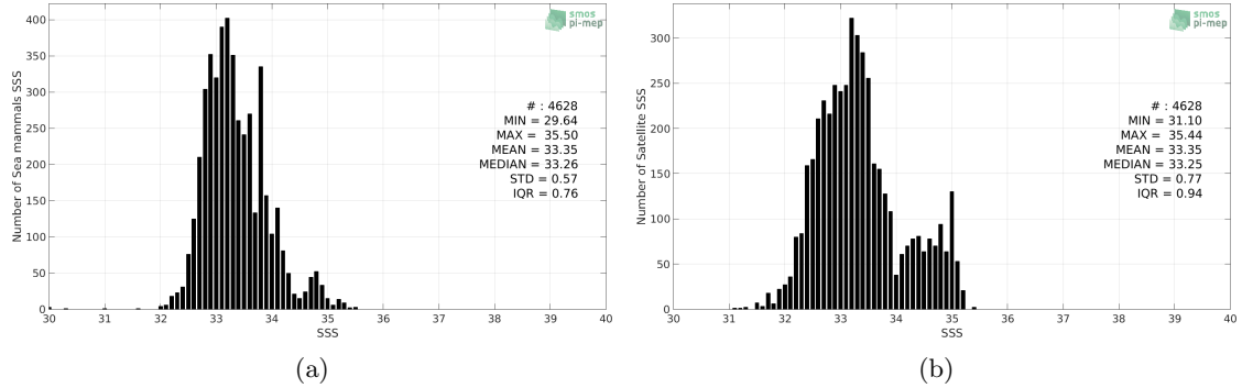
Figure 2: Histograms of SSS from Sea mammals (a) and SMOS-L3-CATDS-CPDC-V317-MONTHLY-25KM (b) considering all match-up pairs per bins of 0.1 over the Mid-Low Latitudes 45N-45S Pi-MEP region and for the full satellite product period.
