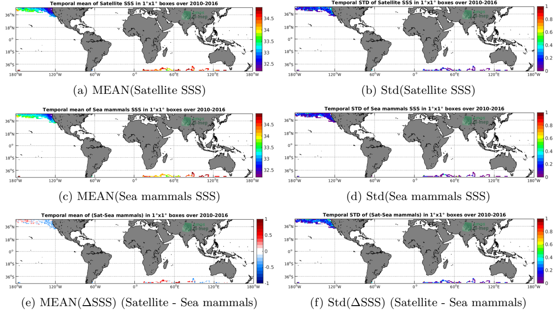
Figure 6: Temporal mean (left) and Std (right) of SSS from SMOS-L3-CATDS-CPDC-V317-MONTHLY-25KM (top), Sea mammals (middle), and of \Delta SSS (Satellite - Sea mammals). Only match-up pairs are used to generate these maps.
