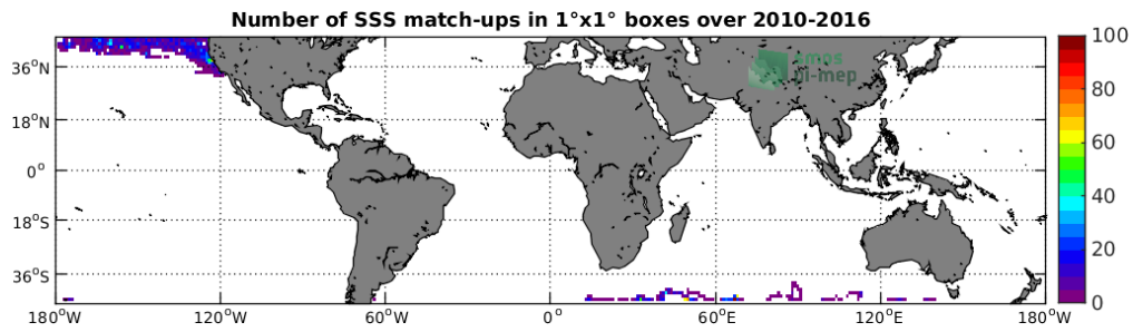
Figure 4: Number of SSS match-ups between Sea mammals SSS and the SMOS-L3-CATDS-CPDC-V317-MONTHLY-25KM SSS product for the Mid-Low Latitudes 45N-45S Pi-MEP region over 1^\circ \times 1^\circ boxes and for the full satellite product period.
