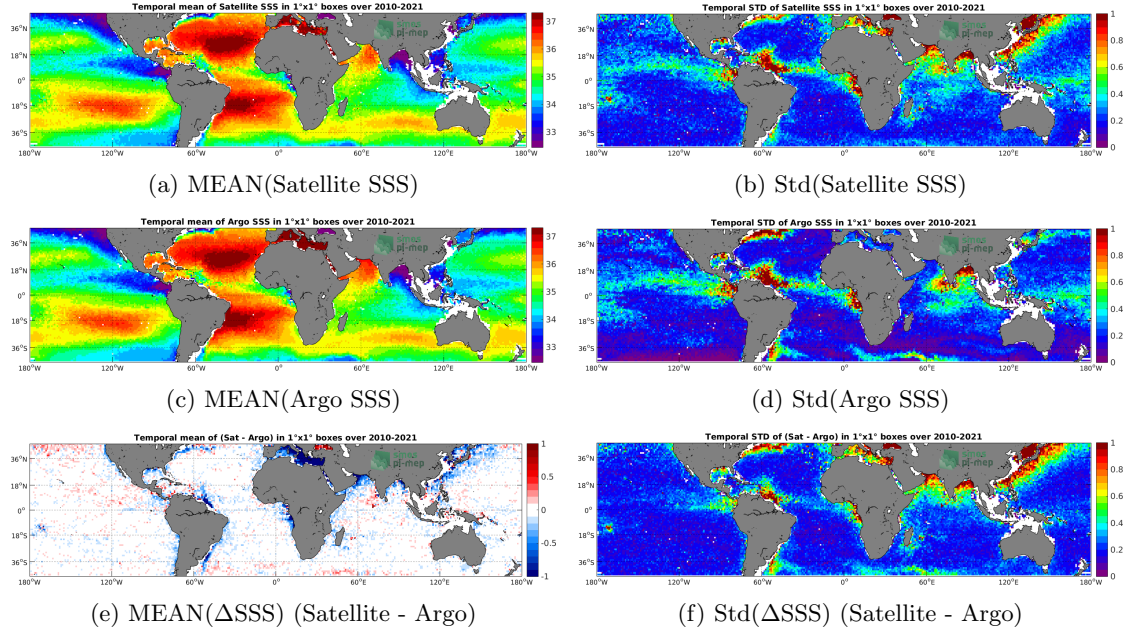
Figure 6: Temporal mean (left) and Std (right) of SSS from SMOS SSS L3 v317 - Monthly - 25 km (CATDS-CPDC) (top), Argo (middle), and of \Delta SSS (Satellite - Argo). Only match-up pairs are used to generate these maps.
