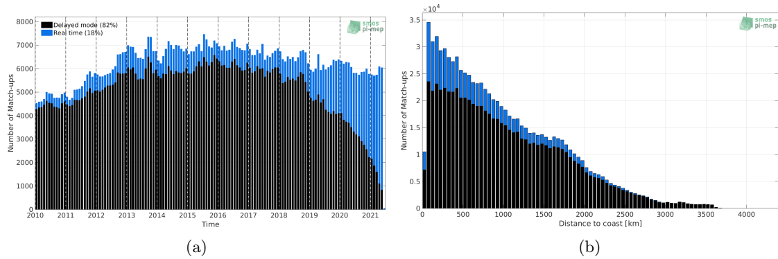
Figure 1: Number of match-ups between Argo and SMOS SSS L3 v317 - Monthly - 25 km (CATDS-CPDC) SSS as a function of time (a) and as function of the distance to coast (b) over the Mid-Low Latitudes 45N-45S Pi-MEP region and for the full satellite product period.
