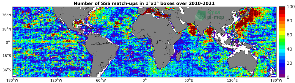
Figure 4: Number of SSS match-ups between Argo SSS and the SMOS SSS L3 v317 - Monthly - 25 km (CATDS-CPDC) SSS product for the Mid-Low Latitudes 45N-45S Pi-MEP region over 1^\circ \times 1^\circ boxes and for the full satellite product period.
