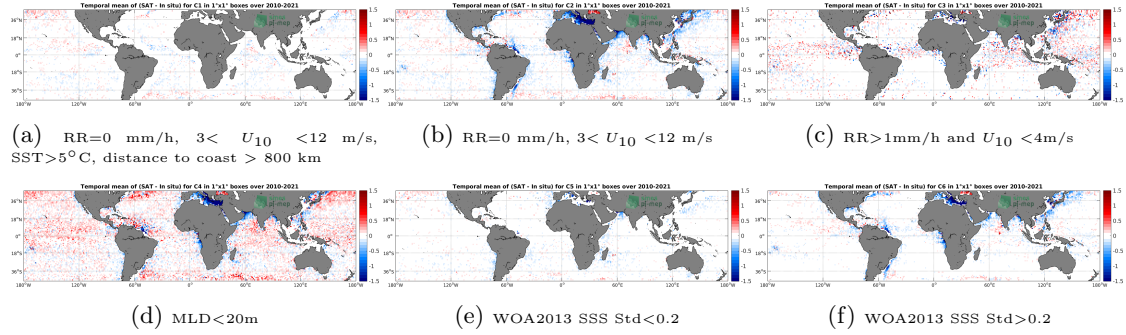
Figure 12: Temporal mean gridded over spatial boxes of size 1^\circ \times 1^\circ of \Delta SSS (SMOS SSS L3 v317 - Monthly - 25 km (CATDS-CPDC) - Argo) for 6 different subdatasets corresponding to: RR=0 mm/h, 3 < U_{10} < 12 m/s, SST > 5^\circ C , distance to coast > 800 km (a), RR=0 mm/h, 3 < U_{10} < 12 m/s (b), RR > 1 mm/h and U_{10} < 4 m/s (c), MLD < 20 m (d), WOA2013 SSS Std < 0.2 (e), WOA2013 SSS Std > 0.2 (f).
