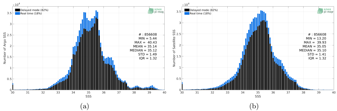
Figure 2: Histograms of SSS from Argo (a) and SMOS SSS L3 v317 - Monthly - 25 km (CATDS-CPDC) (b) considering all match-up pairs per bins of 0.1 over the Mid-Low Latitudes 45N-45S Pi-MEP region and for the full satellite product period.
