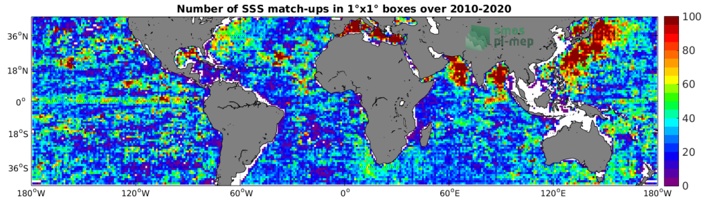
Figure 4: Number of SSS match-ups between Argo SSS and the SMOS L3 v317 - Monthly - 25 km (CATDS-CPDC) SSS product for the Mid-Low Latitudes 45N-45S Pi-MEP region over 1^\circ \times 1^\circ boxes and for the full satellite product period.
