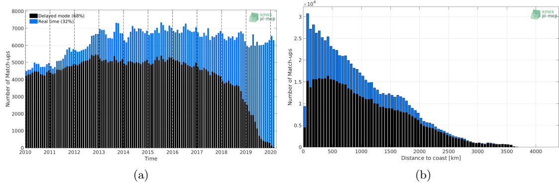
Figure 1: Number of match-ups between Argo and SMOS L3 v317 - Monthly - 25 km (CATDS-CPDC) SSS as a function of time (a) and as function of the distance to coast (b) over the Mid-Low Latitudes 45N-45S Pi-MEP region and for the full satellite product period.
