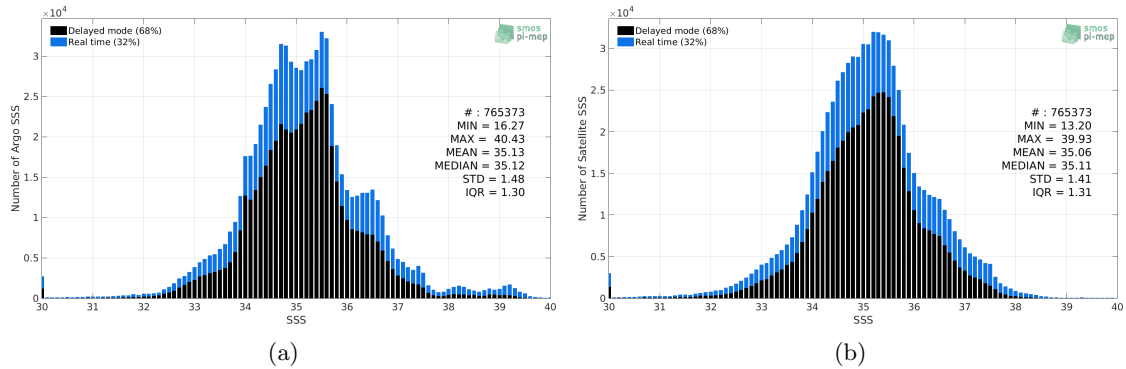
Figure 2: Histograms of SSS from Argo (a) and SMOS L3 v317 - Monthly - 25 km (CATDS-CPDC) (b) considering all match-up pairs per bins of 0.1 over the Mid-Low Latitudes 45N-45S Pi-MEP region and for the full satellite product period.
