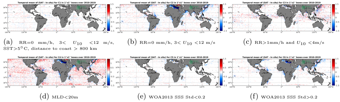
Figure 12: Temporal mean gridded over spatial boxes of size 1^\circ \times 1^\circ of \Delta SSS (SMOS-L3-CATDS-CPDC-V317-MONTHLY-25KM - Argo) for 6 different subdatasets corresponding to: RR=0 mm/h, 3 < U_{10} < 12 m/s, SST > 5^\circ C , distance to coast > 800 km (a), RR=0 mm/h, 3 < U_{10} < 12 m/s (b), RR > 1 mm/h and U_{10} < 4 m/s (c), MLD < 20 m (d), WOA2013 SSS Std < 0.2 (e), WOA2013 SSS Std > 0.2 (f).
