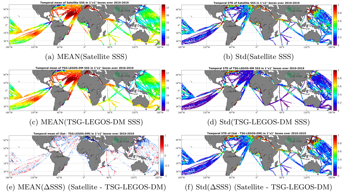
Figure 6: Temporal mean (left) and Std (right) of SSS from SMOS L3 v317 - 10 Days - 25 km (CATDS-CPDC) (top), TSG-LEGOS-DM (middle), and of \Delta SSS (Satellite - TSG-LEGOS-DM). Only match-up pairs are used to generate these maps.
