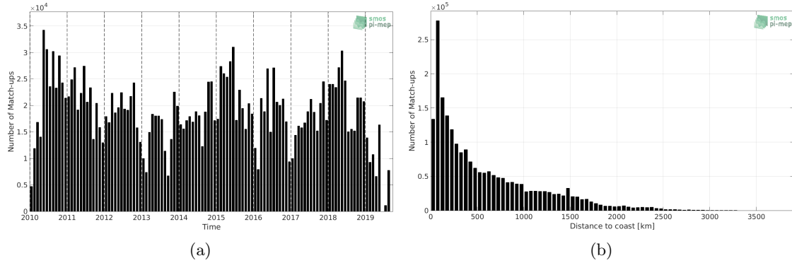
Figure 1: Number of match-ups between TSG-LEGOS-DM and SMOS L3 v317 - 10 Days - 25 km (CATDS-CPDC) SSS as a function of time (a) and as function of the distance to coast (b) over the Mid-Low Latitudes 45N-45S Pi-MEP region and for the full satellite product period.
