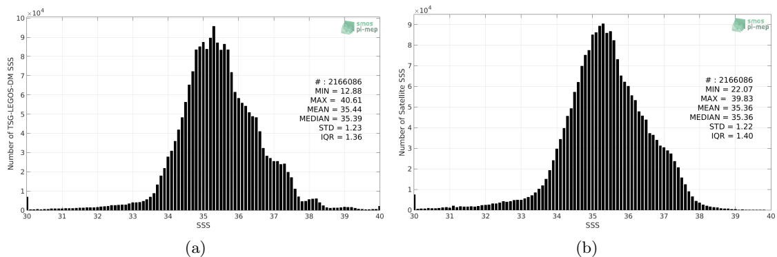
Figure 2: Histograms of SSS from TSG-LEGOS-DM (a) and SMOS L3 v317 - 10 Days - 25 km (CATDS-CPDC) (b) considering all match-up pairs per bins of 0.1 over the Mid-Low Latitudes 45N-45S Pi-MEP region and for the full satellite product period.
