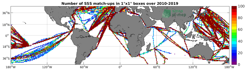
Figure 4: Number of SSS match-ups between TSG-LEGOS-DM SSS and the SMOS L3 v317 - 10 Days - 25 km (CATDS-CPDC) SSS product for the Mid-Low Latitudes 45N-45S Pi-MEP region over 1^\circ \times 1^\circ boxes and for the full satellite product period.
