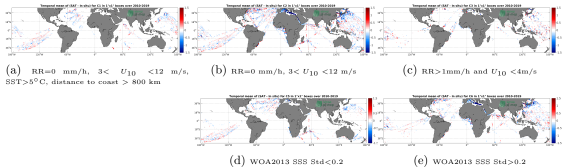
Figure 12: Temporal mean gridded over spatial boxes of size 1^\circ \times 1^\circ of \Delta SSS (SMOS L3 v317 - 10 Days - 25 km (CATDS-CPDC) - TSG-LEGOS-DM) for 5 different subdatasets corresponding to:RR=0 mm/h, 3 < U_{10} < 12 m/s, SST >5^\circ C, distance to coast > 800 km (a), RR=0 mm/h, 3 < U_{10} < 12 m/s (b), RR >1 mm/h and U_{10} < 4 m/s (c), WOA2013 SSS Std <0.2 (d), WOA2013 SSS Std >0.2 (e).
