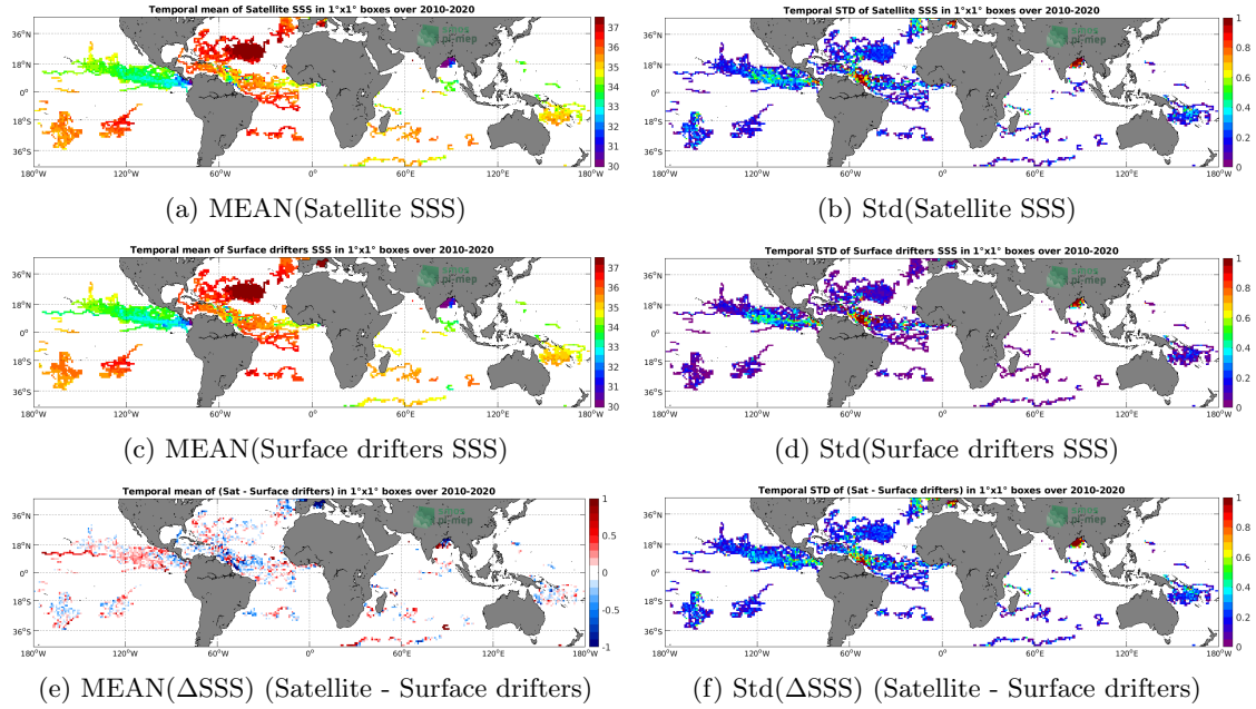
Figure 5: Temporal mean (left) and Std (right) of SSS from SMOS SSS L3 v317 - 10 Days - 25 km (CATDS-CPDC) (top), Surface drifters (middle), and of \Delta SSS (Satellite - Surface drifters). Only match-up pairs are used to generate these maps.
