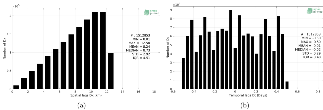
Figure 4: Histograms of the spatial (a) and temporal (b) lags between the location/time of the Surface drifters measurement and the date of the corresponding SMOS SSS L3 v317 - 10 Days - 25 km (CATDS-CPDC) SSS pixel.
