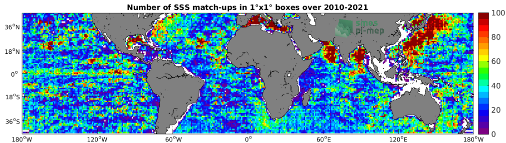
Figure 4: Number of SSS match-ups between Argo SSS and the SMOS SSS L3 v317 - 10 Days - 25 km (CATDS-CPDC) SSS product for the Mid-Low Latitudes 45N-45S Pi-MEP region over 1^\circ \times 1^\circ boxes and for the full satellite product period.
