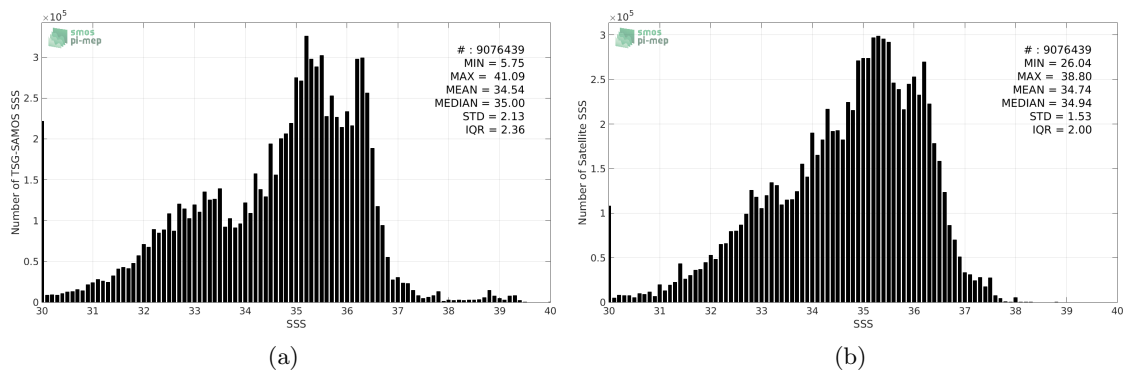
Figure 2: Histograms of SSS from TSG-SAMOS (a) and SMOS-L3-CATDS-CPDC-V3-MONTHLY-25KM (b) considering all match-up pairs per bins of 0.1 over the Mid-Low Latitudes 45N-45S Pi-MEP region and for the full satellite product period.
