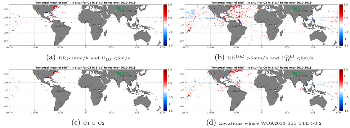
Figure 12: Temporal mean gridded over spatial boxes of size 1^\circ \times 1^\circ of \Delta SSS (SMOS-L3-CATDS-CPDC-V3-MONTHLY-25KM - TSG-SAMOS) for 4 different subdatasets corresponding to: RR > 1\text{mm/h} and U_{10} < 5\text{m/s} (a), RR^{10d} > 5\text{mm/h} and U_{10}^{10d} < 5\text{m/s} (b), C1 U C2 (c), Locations where WOA2013 SSS STD > 0.2 (d).
