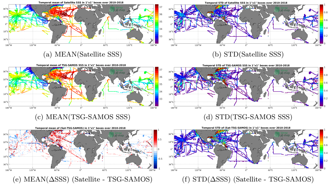
Figure 6: Temporal mean (left) and STD (right) of SSS from SMOS-L3-CATDS-CPDC-V3-MONTHLY-25KM (top), TSG-SAMOS (middle), and of \Delta SSS (Satellite - TSG-SAMOS). Only match-up pairs are used to generate these maps.
