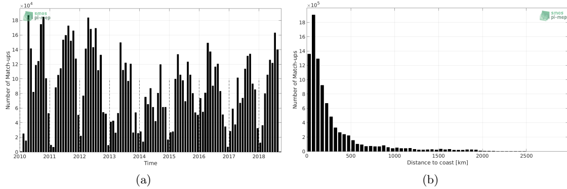
Figure 1: Number of match-ups between TSG-SAMOS and SMOS-L3-CATDS-CPDC-V3-MONTHLY-25KM SSS as a function of time (a) and as function of the distance to coast (b) over the Mid-Low Latitudes 45N-45S Pi-MEP region and for the full satellite product period.
