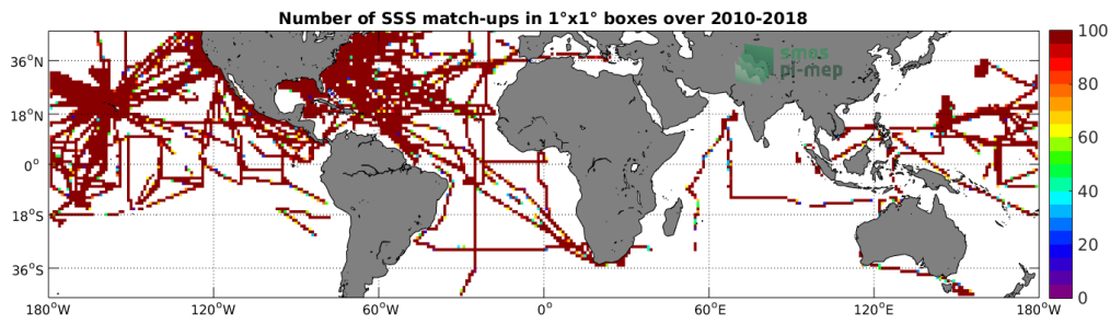
Figure 4: Number of SSS match-ups between TSG-SAMOS SSS and the SMOS-L3-CATDS-CPDC-V3-MONTHLY-25KM SSS product for the Mid-Low Latitudes 45N-45S Pi-MEP region over 1^\circ \times 1^\circ boxes and for the full satellite product period.
