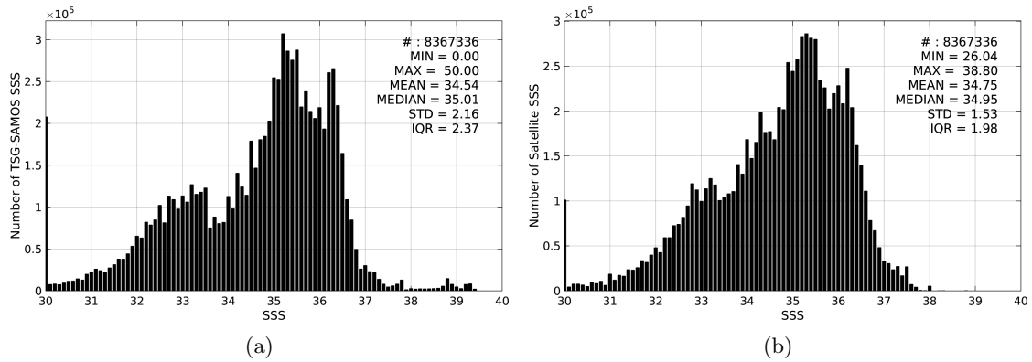
Figure 2: Histograms of SSS from TSG-SAMOS (a) and SMOS-L3-CATDS-CPDC-V3-MONTHLY-25KM (b) considering all match-up pairs per bins of 0.1 over the Mid-Low Latitudes 45N-45S Pi-MEP region and for the full satellite product period.
