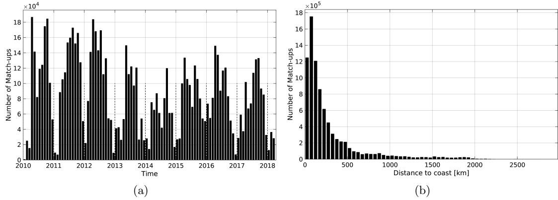
Figure 1: Number of match-ups between TSG-SAMOS and SMOS-L3-CATDS-CPDC-V3-MONTHLY-25KM SSS as a function of time (a) and as function of the distance to coast (b) over the Mid-Low Latitudes 45N-45S Pi-MEP region and for the full satellite product period.
