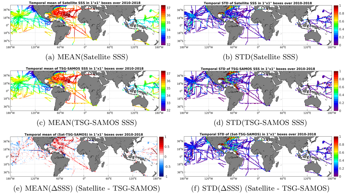
Figure 6: Temporal mean (left) and STD (right) of SSS from SMOS-L3-CATDS-CPDC-V3-MONTHLY-25KM (top), TSG-SAMOS (middle), and of \Delta SSS (Satellite - TSG-SAMOS). Only match-up pairs are used to generate these maps.
