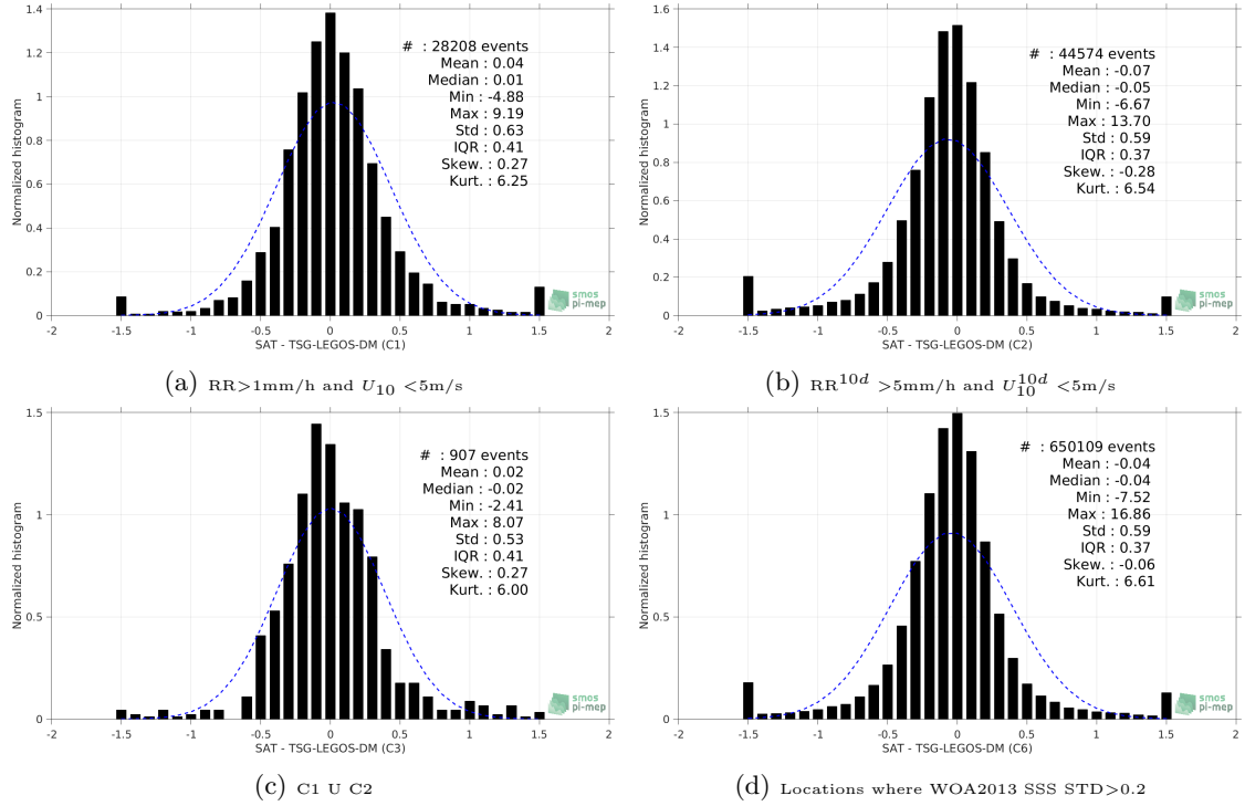
Figure 13: Normalized histogram of \Delta SSS (SMOS-L3-CATDS-CPDC-V3-MONTHLY-25KM - TSG-LEGOS-DM) for 6 different subdatasets corresponding to: RR > 1mm/h and U_{10} < 5 m/s (a), RR^{10d} > 5 mm/h and U_{10}^{10d} < 5 m/s (b), C1 U C2 (c), Locations where WOA2013 SSS STD > 0.2 (d).
