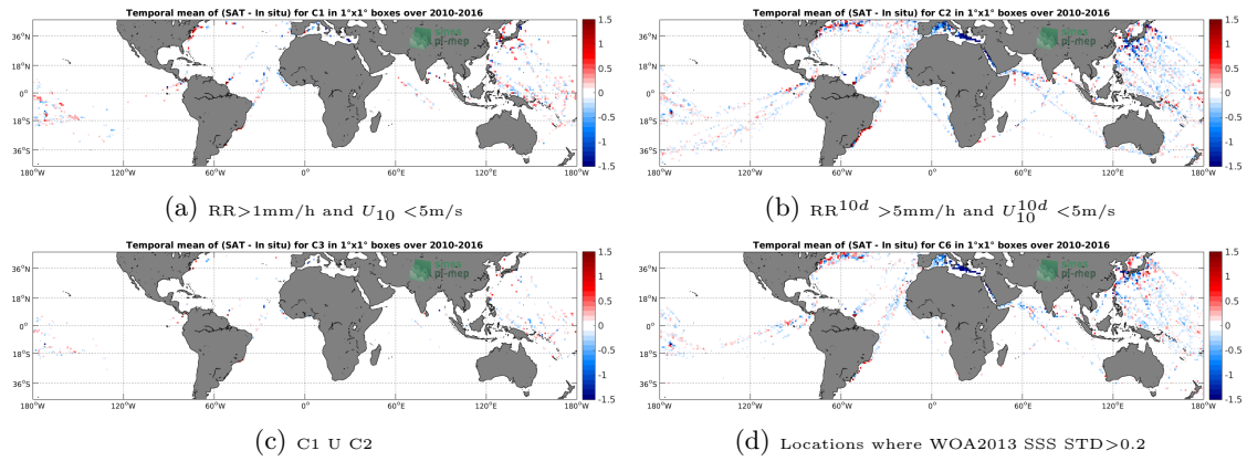
Figure 12: Temporal mean gridded over spatial boxes of size 1^\circ \times 1^\circ of \Delta SSS (SMOS-L3-CATDS-CPDC-V3-MONTHLY-25KM - TSG-LEGOS-DM) for 4 different subdatasets corresponding to: RR > 1\text{mm/h} and U_{10} < 5\text{m/s} (a), RR^{10d} > 5\text{mm/h} and U_{10}^{10d} < 5\text{m/s} (b), C1 U C2 (c), Locations where WOA2013 SSS STD > 0.2 (d).
