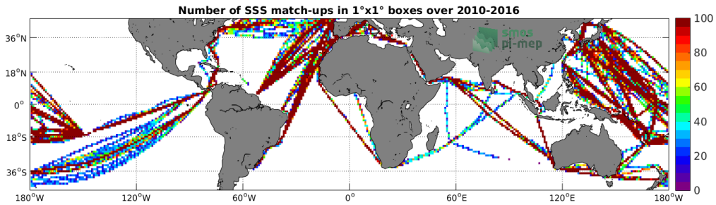
Figure 4: Number of SSS match-ups between TSG-LEGOS-DM SSS and the SMOS-L3-CATDS-CPDC-V3-MONTHLY-25KM SSS product for the Mid-Low Latitudes 45N-45S Pi-MEP region over 1^\circ \times 1^\circ boxes and for the full satellite product period.
