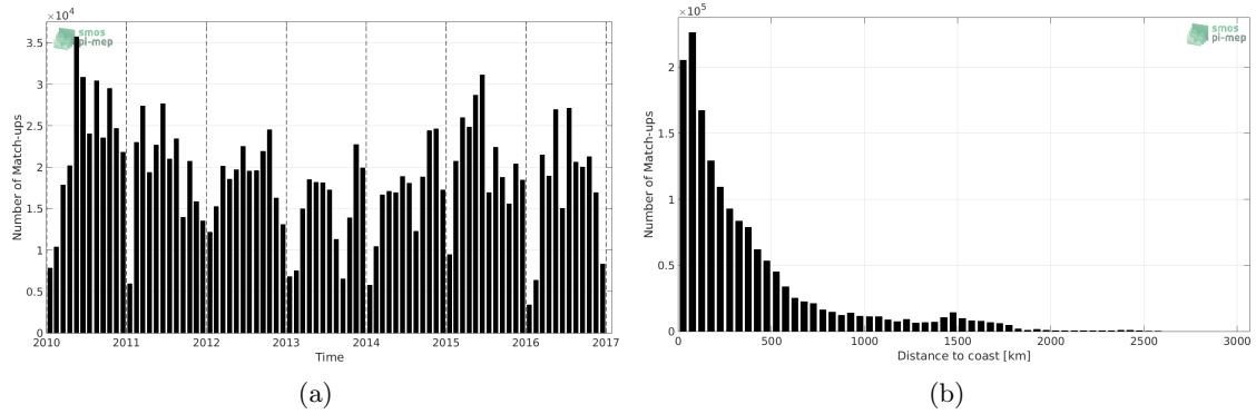
Figure 1: Number of match-ups between TSG-LEGOS-DM and SMOS-L3-CATDS-CPDC-V3-MONTHLY-25KM SSS as a function of time (a) and as function of the distance to coast (b) over the Mid-Low Latitudes 45N-45S Pi-MEP region and for the full satellite product period.
