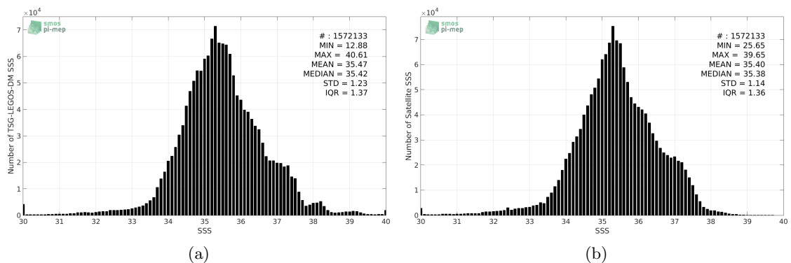
Figure 2: Histograms of SSS from TSG-LEGOS-DM (a) and SMOS-L3-CATDS-CPDC-V3-MONTHLY-25KM (b) considering all match-up pairs per bins of 0.1 over the Mid-Low Latitudes 45N-45S Pi-MEP region and for the full satellite product period.
