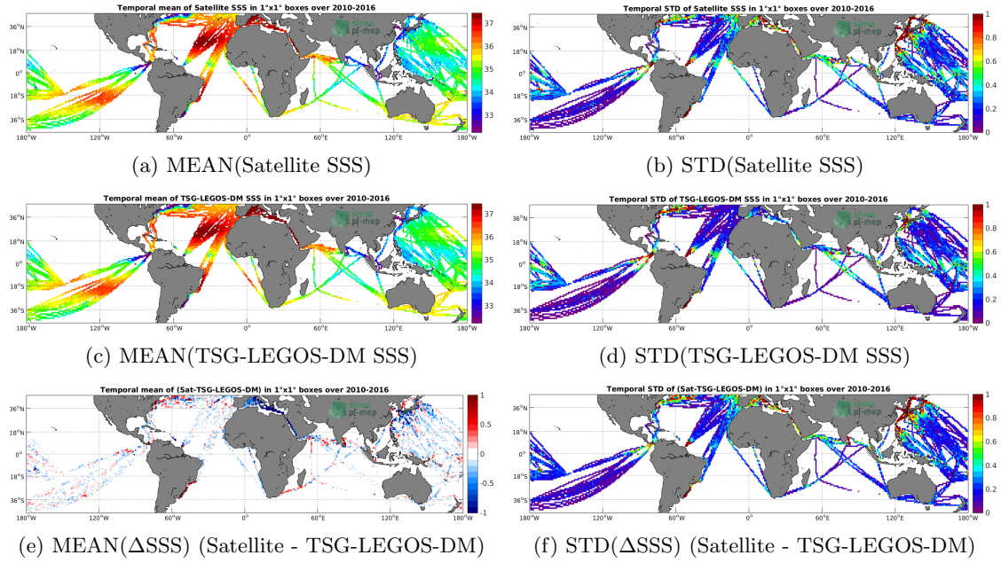
Figure 6: Temporal mean (left) and STD (right) of SSS from SMOS-L3-CATDS-CPDC-V3-MONTHLY-25KM (top), TSG-LEGOS-DM (middle), and of \Delta SSS (Satellite - TSG-LEGOS-DM). Only match-up pairs are used to generate these maps.
