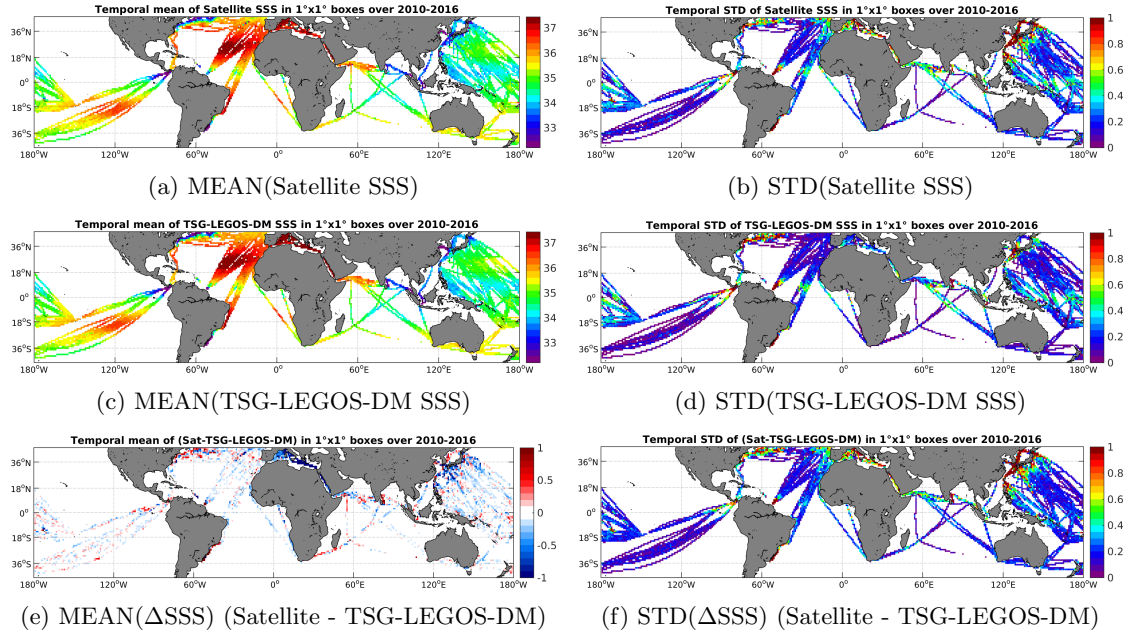
Figure 6: Temporal mean (left) and STD (right) of SSS from SMOS-L3-CATDS-CPDC-V3-MONTHLY-25KM (top), TSG-LEGOS-DM (middle), and of \Delta SSS (Satellite - TSG-LEGOS-DM). Only match-up pairs are used to generate these maps.
