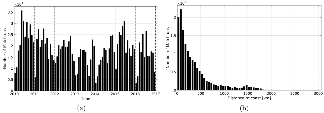
Figure 1: Number of match-ups between TSG-LEGOS-DM and SMOS-L3-CATDS-CPDC-V3-MONTHLY-25KM SSS as a function of time (a) and as function of the distance to coast (b) over the Mid-Low Latitudes 45N-45S Pi-MEP region and for the full satellite product period.
