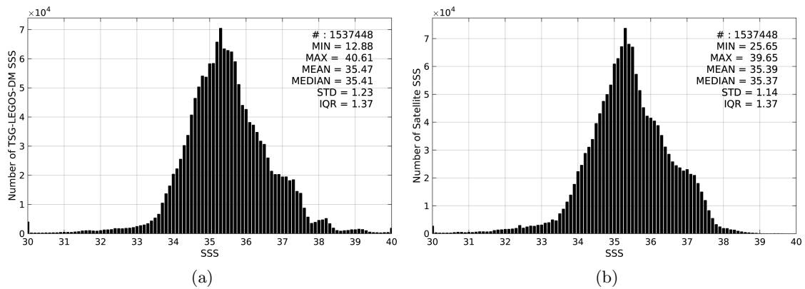
Figure 2: Histograms of SSS from TSG-LEGOS-DM (a) and SMOS-L3-CATDS-CPDC-V3-MONTHLY-25KM (b) considering all match-up pairs per bins of 0.1 over the Mid-Low Latitudes 45N-45S Pi-MEP region and for the full satellite product period.
