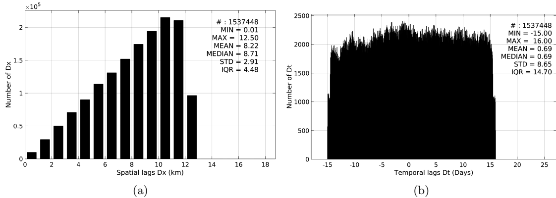
Figure 5: Histograms of the spatial (a) and temporal (b) lags between the time of the TSG-LEGOS-DM measurements and the date of the corresponding SMOS-L3-CATDS-CPDC-V3-MONTHLY-25KM SSS product.
