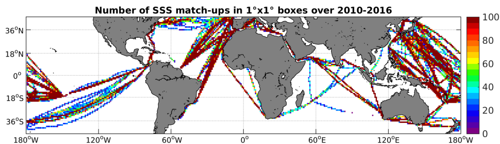
Figure 4: Number of SSS match-ups between TSG-LEGOS-DM SSS and the SMOS-L3-CATDS-CPDC-V3-MONTHLY-25KM SSS product for the Mid-Low Latitudes 45N-45S Pi-MEP region over 1°x1° boxes and for the full satellite product period.
