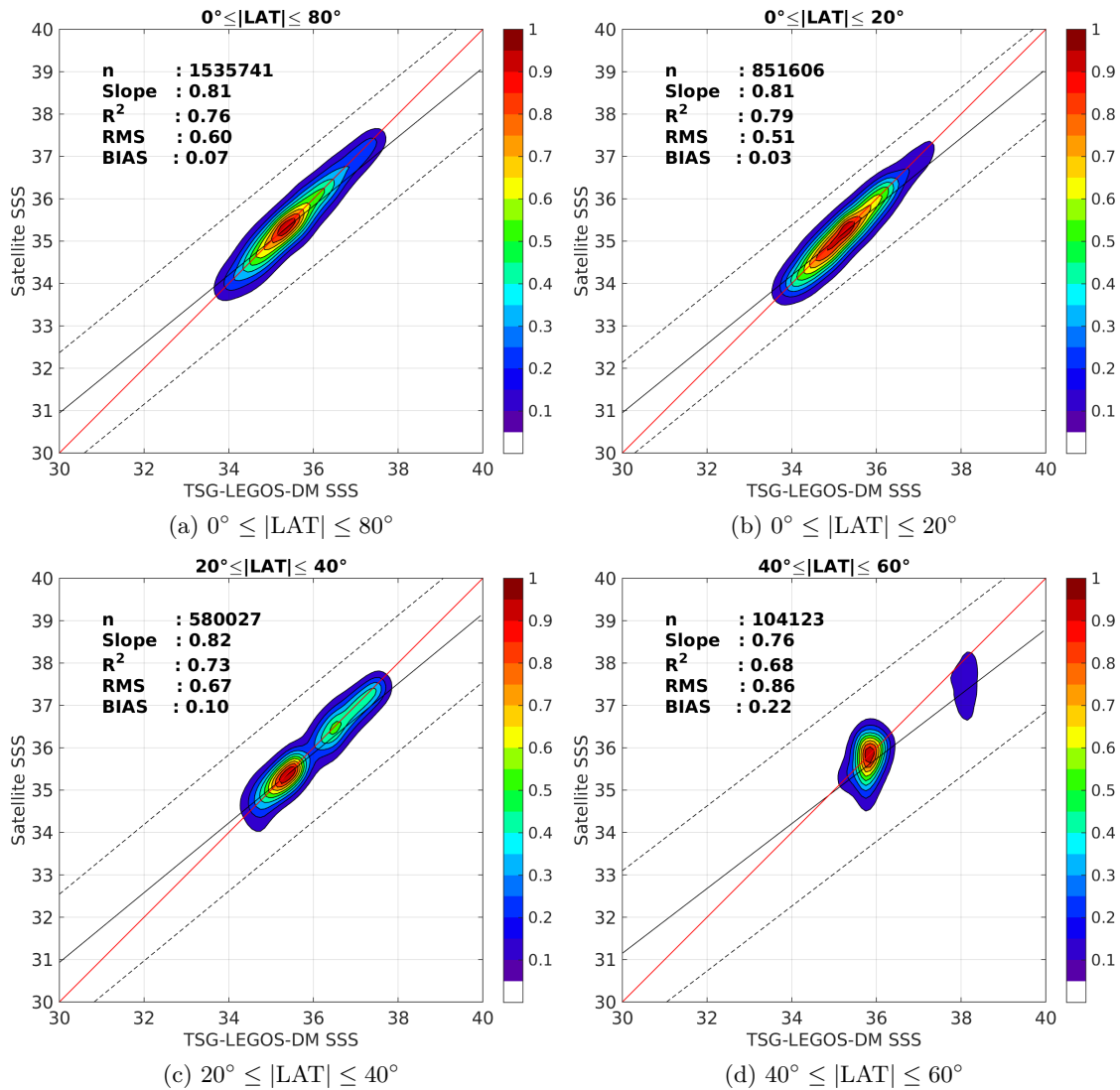
Figure 9: Contour maps of the concentration of SMOS-L3-CATDS-CPDC-V3-MONTHLY-25KM SSS (y-axis) versus TSG-LEGOS-DM SSS (x-axis) at match-up pairs for different latitude bands. For each plot, the red line shows x=y . The black thin and dashed lines indicate a linear fit through the data cloud and the \pm 95\% confidence levels, respectively. The number match-up pairs n , the slope and R^2 coefficient of the linear fit, the root mean square (RMS) and the mean bias between satellite and in situ data are indicated for each latitude band in each plots.
