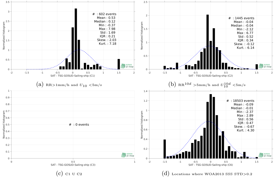
Figure 13: Normalized histogram of \Delta SSS (SMOS-L3-CATDS-CPDC-V3-MONTHLY-25KM - TSG-GOSUD-Sailing-ship) for 6 different subdatasets corresponding to: RR > 1\text{mm/h} and U_{10} < 5\text{m/s} (a), RR^{10d} > 5\text{mm/h} and U_{10}^{10d} < 5\text{m/s} (b), C1 U C2 (c), Locations where WOA2013 SSS STD > 0.2 (d).
