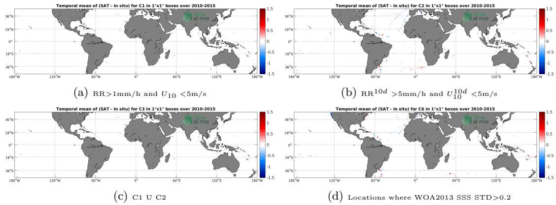
Figure 12: Temporal mean gridded over spatial boxes of size 1^\circ \times 1^\circ of \Delta SSS (SMOS-L3-CATDS-CPDC-V3-MONTHLY-25KM - TSG-GOSUD-Sailing-ship) for 4 different subdatasets corresponding to: RR > 1\text{mm/h} and U_{10} < 5\text{m/s} (a), RR^{10d} > 5\text{mm/h} and U_{10}^{10d} < 5\text{m/s} (b), C1 U C2 (c), Locations where WOA2013 SSS STD > 0.2 (d).
