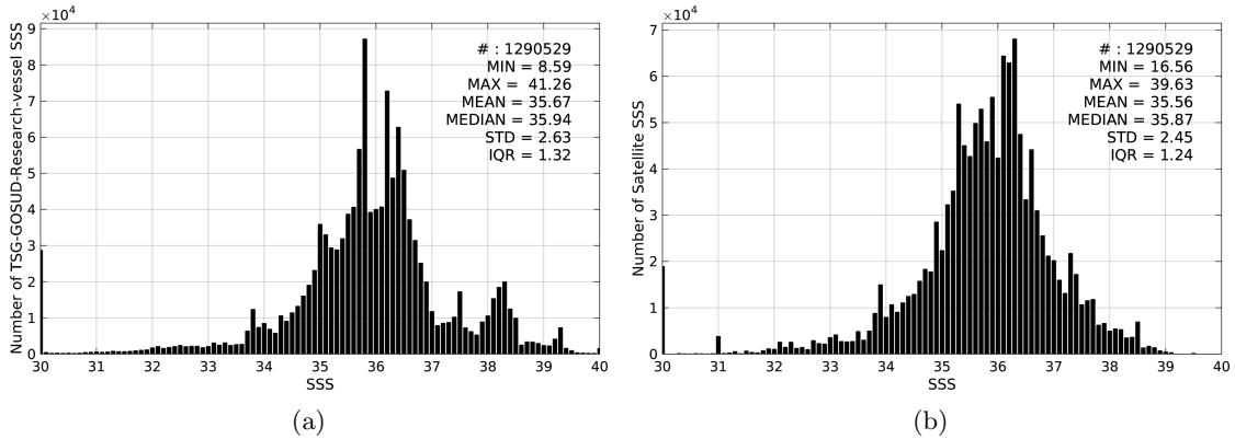
Figure 2: Histograms of SSS from TSG-GOSUD-Research-vessel (a) and SMOS-L3-CATDS-CPDC-V3-MONTHLY-25KM (b) considering all match-up pairs per bins of 0.1 over the Mid-Low Latitudes 45N-45S Pi-MEP region and for the full satellite product period.
