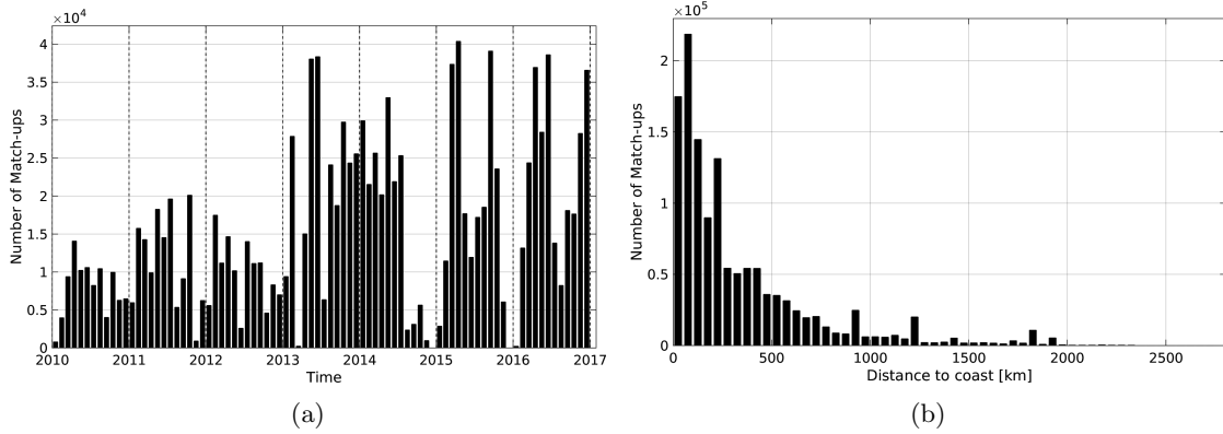
Figure 1: Number of match-ups between TSG-GOSUD-Research-vessel and SMOS-L3-CATDS-CPDC-V3-MONTHLY-25KM SSS as a function of time (a) and as function of the distance to coast (b) over the Mid-Low Latitudes 45N-45S Pi-MEP region and for the full satellite product period.
