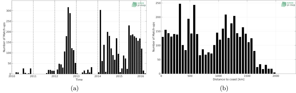
Figure 1: Number of match-ups between Sea mammals and SMOS-L3-CATDS-CPDC-V3-MONTHLY-25KM SSS as a function of time (a) and as function of the distance to coast (b) over the Mid-Low Latitudes 45N-45S Pi-MEP region and for the full satellite product period.
