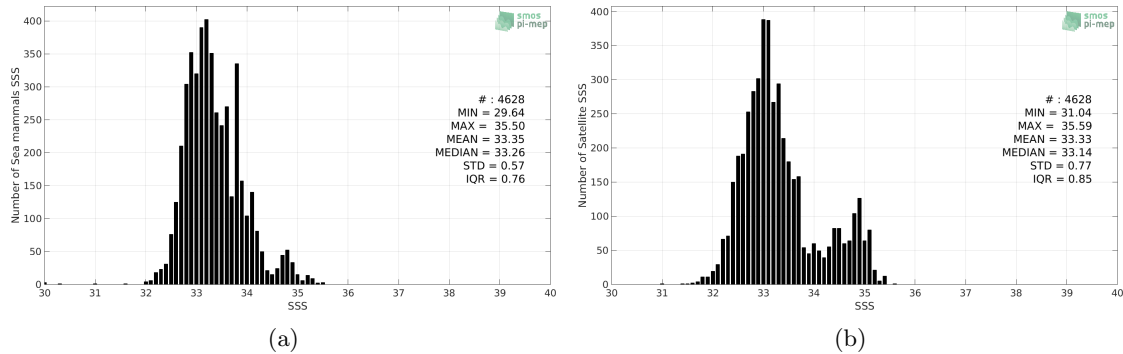
Figure 2: Histograms of SSS from Sea mammals (a) and SMOS-L3-CATDS-CPDC-V3-MONTHLY-25KM (b) considering all match-up pairs per bins of 0.1 over the Mid-Low Latitudes 45N-45S Pi-MEP region and for the full satellite product period.
