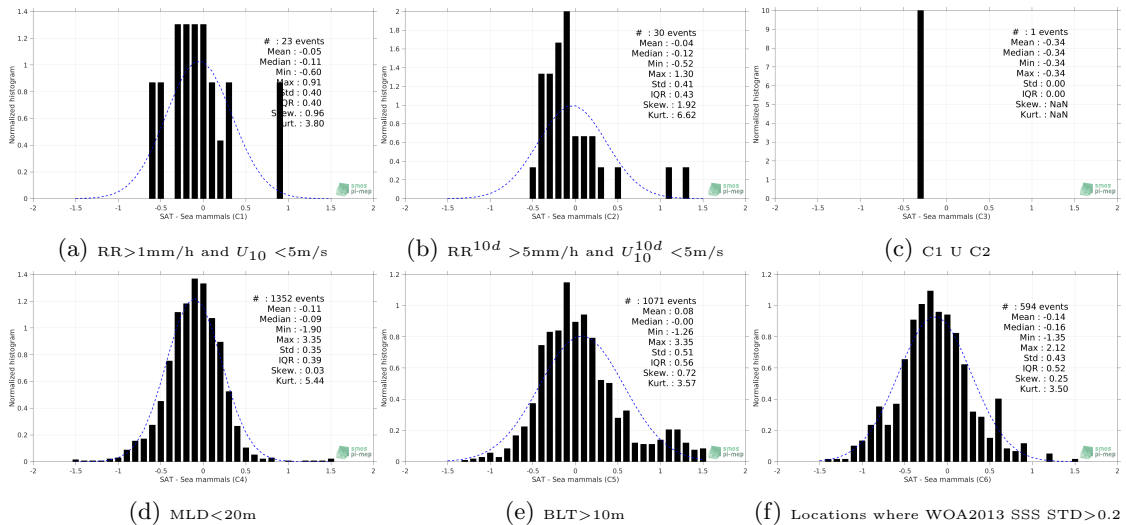
Figure 13: Normalized histogram of \Delta SSS (SMOS-L3-CATDS-CPDC-V3-MONTHLY-25KM - Sea mammals) for 6 different subdatasets corresponding to: RR>1mm/h and U_{10} < 5m/s (a), RR^{10d} > 5mm/h and U_{10}^{10d} < 5m/s (b), C1 U C2 (c),MLD<20m (d),BLT>10m (e),Locations where WOA2013 SSS STD>0.2 (f).
