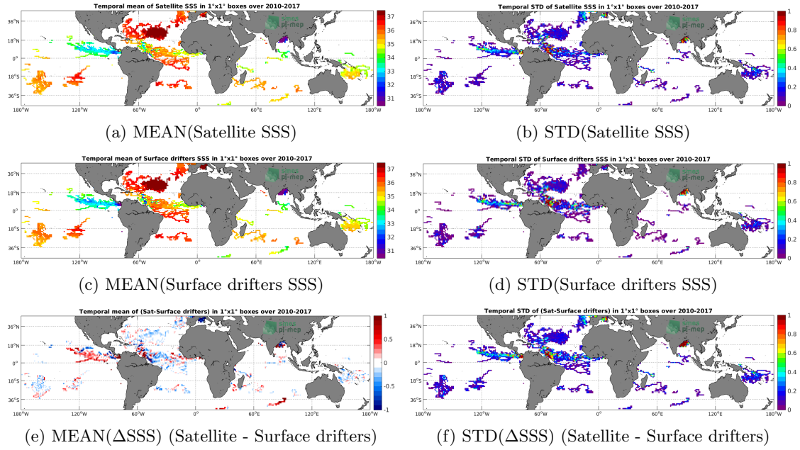
Figure 5: Temporal mean (left) and STD (right) of SSS from SMOS-L3-CATDS-CPDC-V3-MONTHLY-25KM (top), Surface drifters (middle), and of \Delta SSS (Satellite - Surface drifters). Only match-up pairs are used to generate these maps.
